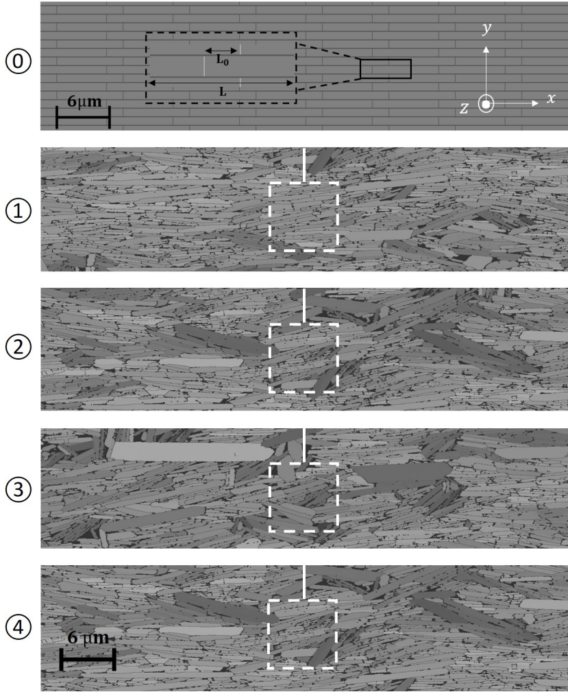
Fig. 1: The five microstructures used in our simulations a) The regular brick and mortar microstructure (M0) used in [14] and a close-up of the overlap region. b) Index quality map resulting from EBSD analysis of a nacre-like alumina sample showing the four images (1-4) that were used in DEM simulations to generate four notched numerical microstructures M1-M4. The dashed white squares highlight the zones ahead of the crack tip used to compute the local microstructure parameters reported in Tab. 2.
