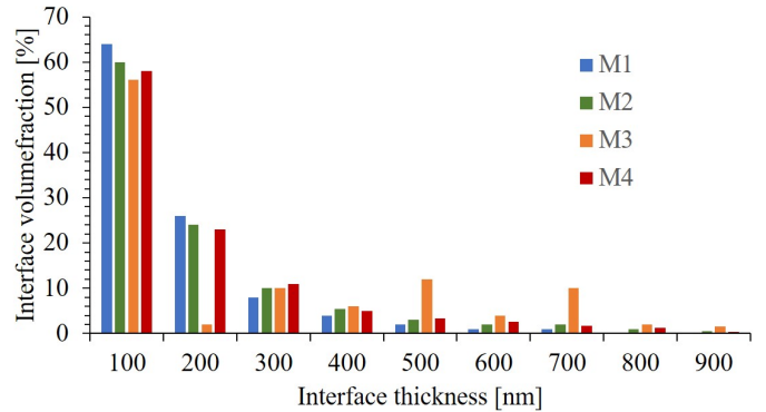
Fig. 2: Histogram of interfaces thickness for the EBSD microstructures, showing the occurrence of thicker interfaces in M3.
