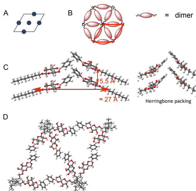
Figure 6. Representation of the hexagonal packing characterized by SAXS for 1e . A: distribution of 5 dimers (6 molecules) within the unit cell; B: self-assembly of dimers within the hexagonal phase and global shape of the dimer; C: self-assembly of 4 molecules and herringbone packing; D: self-assembly of 10 molecules within the unit cell.
