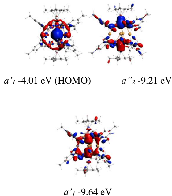
Figure 5: The three occupied orbitals of 2 of large 4s character and responsible for metal-metal bonding in the [Cu 10 Zn 2 ] core.
