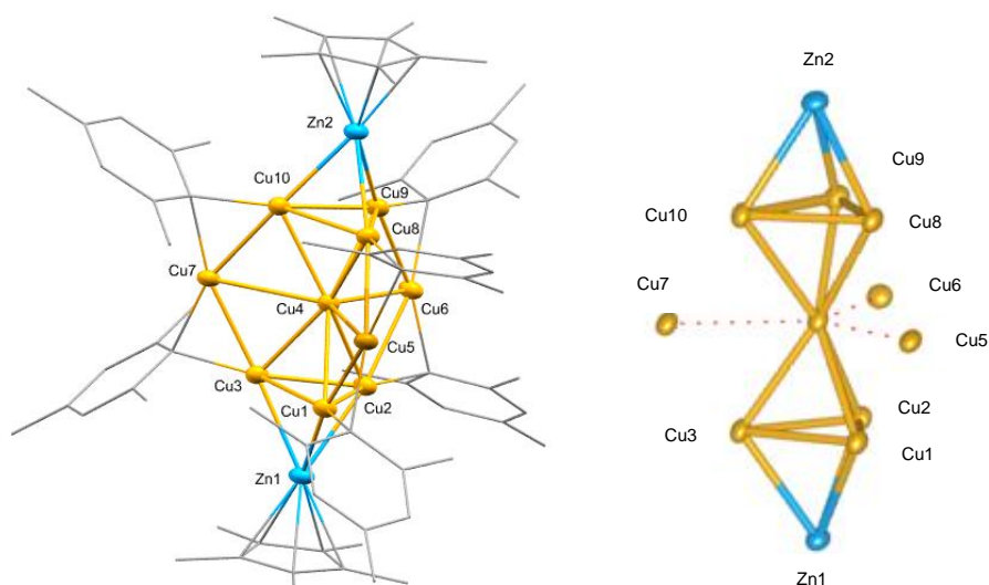
Figure 3: Left: Molecular structure of 2 in the solid state as determined by SC-XRD. Thermal ellipsoids are shown at the 50 % probability level, hydrogen atoms, co-crystallized solvent molecules and disordered groups are not shown for clarity and ligands are simplified as wireframes. Selected interatomic bond distances [Å] and angles [°]: Cu4-Cu10: 2.4617(8), Cu1-Cu5: 2.4223(7), Cu4-Cu3: 2.4566(7), Cu4-Cu7: 2.7662(8), Cu10-Zn2: 2.4659(8), Cu3-Zn1: 2.4528(8), Cu10-Zn2: 2.4658(7), Cu3-Zn1: 2.4526(7), Cu7-C bridging mesityl : 2.030(4), Cu3-C bridging mesityl : 2.012(4), Zn1-Cp* centroid : 1.91, Zn2-Cp* centroid : 1.92, Cu7-C bridging mesityl -Cu3: 52.54(13), Cu10-Cu4-Cu8: 59.85(2), Cu7-Cu4-Cu6: 118.60(2); Cu10-Zn2-Cu8: 59.30(2). Right: Cluster core geometry of 2 (Cu = orange, Zn = blue). Cu-Cu bonds illustrated in orange, Cu-Zn bonds illustrated in orange-blue.
