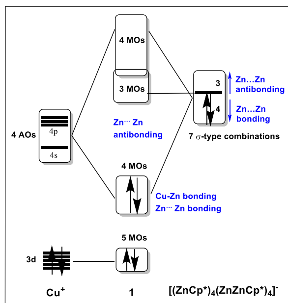
Figure 2: Simplified MO diagram sketching the interaction of the Cu valence AOs with the combinations of the \sigma -type frontier orbitals of the ZnCp* and ZnZnCp* fragments in 1 . For the sake of simplicity Cu is considered in its +I oxidation state, making the whole ligand sphere an 8-electron donor system.
