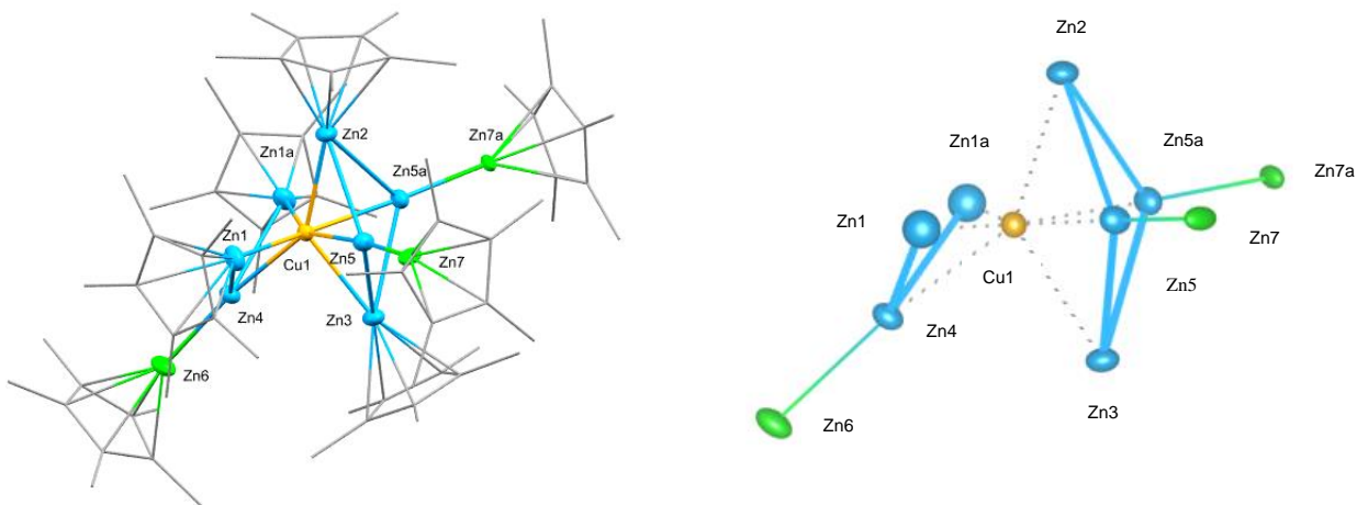
Figure 1: Left: Molecular structure of 1 in the solid state as determined by SC-XRD. Thermal ellipsoids are shown at the 50 % probability level, hydrogen atoms, co-crystallized solvent molecules and disordered groups are not shown for clarity and ligands are simplified as wireframes. Selected interatomic bond distances [Å] and angles [°]: Cu1-Zn5: 2.3477(3), Cu1-Zn1: 2.335(5), Cu1-Zn2: 2.3997(5), Cu1-Zn4: 2.3662(4), Cu1-Zn3: 2.4136(5), Zn4-Zn6: 2.3686(5), Zn5-Zn7: 2.390(5), Zn2-Zn5: 2.7489(4), Zn1-Zn4: 2.713(6), Zn5-Zn3: 2.7418(4), Cu1-Zn4-Zn6: 173.08(2), Cu1-Zn5-Zn7: 172.0(2). Right: Coordination geometry of Cu (orange) in 1 with Zn in the first (blue) and second coordination sphere (green). Longer Zn-Zn contacts are illustrated in blue, shorter ones as a blue-green gradient line.
