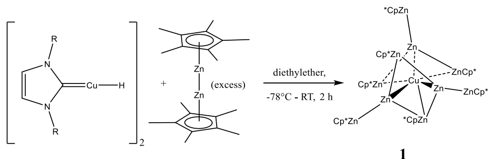
Scheme 1: Synthesis of cluster 1 , [\text{CuZn}_{10}](\text{Cp}^*)_7 = [\text{Cu}(\text{ZnZn}\text{Cp}^*)_3(\text{Zn}\text{Cp}^*)_4] ( \text{R} = 2,6 -diisopropylphenyl). The Cu-Zn connecting lines illustrate short contacts.
