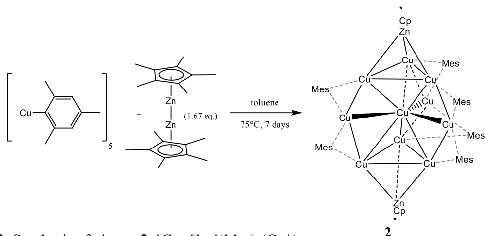
Scheme 2: Synthesis of cluster 2 , [\text{Cu}_{10}\text{Zn}_2](\text{Mes})_6(\text{Cp}^*)_2 .
