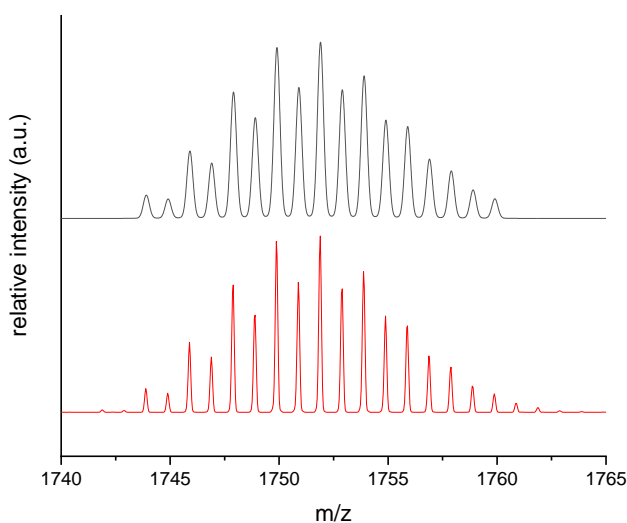
Figure 4: Comparison of the experimental (as determined by positive ion-mode LIFDI-MS; bottom, red) and calculated (top, black) isotopic pattern of [\text{Cu}_{10}\text{Zn}_2]\text{Mes}_6\text{Cp}^*_2 ( 2 ).
