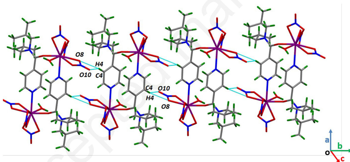
Figure 2. Showing the hydrogen bonding of the dimeric unit with cocrystallized ligand along the c axis forming 1D chains.
