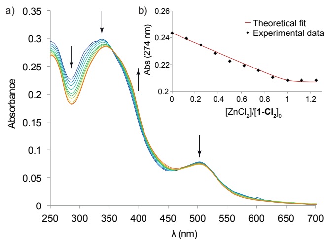
Fig. 2. a) UV-Vis titration of 1-Cl}_2 ( 5.0 \times 10^{-6} \text{ mol}\cdot\text{L}^{-1} ) by \text{ZnCl}_2 in \text{CHCl}_3 . b) Absorption at 274 nm and fitting with a 1:1 binding model.
