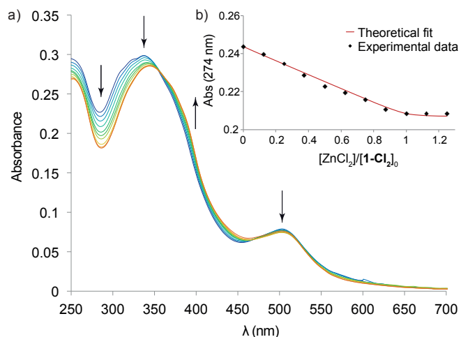
Fig. 2. a) UV-Vis titration of \mathbf{1}\text{-Cl}_2 ( 5.0 \times 10^{-6} \text{ mol}\cdot\text{L}^{-1} ) by \text{ZnCl}_2 in \text{CHCl}_3 . b) Absorption at 274 nm and fitting with a 1:1 binding model.
