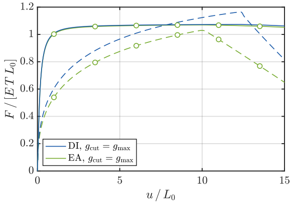
(c) Sticking-dominated peeling: \mu_{\text{EA}} = \mu_{\text{DI}} = 0.05 .
