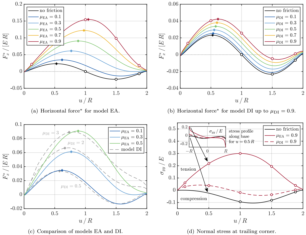
Figure 10: 2D contact of two deformable cylinders: (a) – (c) Horizontal forces* (*: per out-of-plane width) acting on each body for models EA and DI, both with g_{cut} = g_{max} ; asterisks indicate the horizontal displacement at which snap through would occur in a horizontally load-controlled setup; (d) normal stress \sigma_{yy} / E at the (left) trailing corner of the bottom cylinder for the cases from Fig. 9(b) – 9(d); the inset in Fig. (d) shows \sigma_{yy} / E along the base of the lower cylinder for a displacement of u = 0.5 R ; the white dots in Figs. (a) – (d) mark the configurations shown in Fig. 9(b) – 9(d), respectively.
