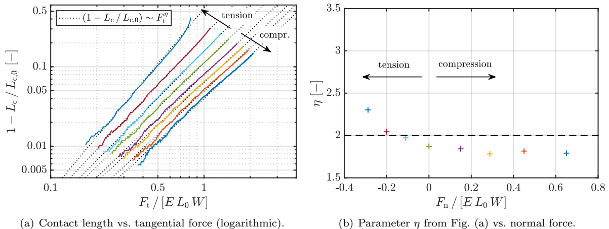
Figure 14: Adhesive friction of a 2D cap: (a) Logarithmic representation of the contact length in dependence of the tangential force as considered in Papangelo et al. (2019); the figure shows the adhesive cases from Fig. 13 with stable (non-vanishing) contact; (b) parameter \eta (fitted from (1 - L_c / L_{c,0}) \sim F_t^\eta , and illustrated in Fig. (a) as dotted lines) versus the normal force.
