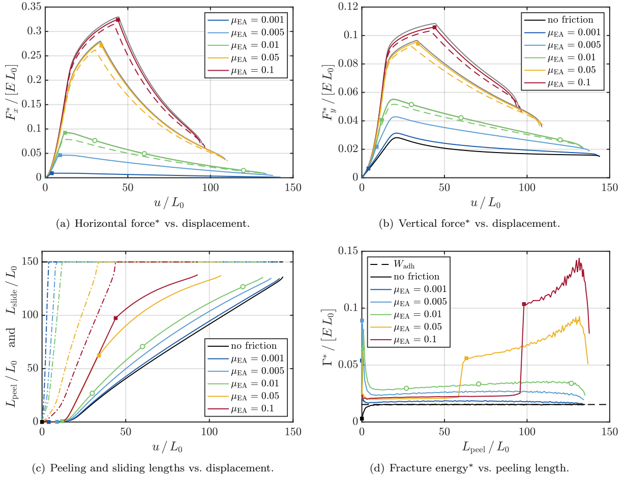
Figure 8: 2D strip peeling: (a) & (b) Horizontal and vertical forces* (*: per out-of-plane width); solid colored lines: model EA with g_{cut} = g_{max} ; dashed colored lines: model EA with g_{cut} = (g_{eq} + g_{max})/2 ; solid gray lines: model DI with \mu_{DI} = \mu_{EA} and g_{cut} = g_{max} ; (c) nominal peeling length L_{peel} (solid) and nominal sliding length L_{slide} (dash-dotted); (d) fracture energy*; the white dots in Figs. (a) – (d) mark the configurations plotted in Fig. 6; the filled squares indicate the onset of full sliding rounded to next integer value of u .
