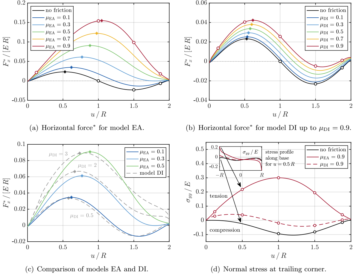
Figure 10 2D contact of two deformable cylinders: (a) – (c) Horizontal forces* (*: per out-of-plane width) acting on each body for models EA and DI, both with g_{\text{cut}} = g_{\text{max}} ; asterisks indicate the horizontal displacement at which snap through would occur in a horizontally load-controlled setup; (d) normal stress \sigma_{yy} / E at the (left) trailing corner of the bottom cylinder for the cases from Fig. 9(b) – 9(d); the inset in Fig. (d) shows \sigma_{yy} / E along the base of the lower cylinder for a displacement of u = 0.5R ; the dots in Figs. (a) – (d) mark the configurations shown in Fig. 9(b) – 9(d), respectively.
