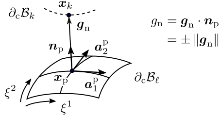
Figure 1 Closest projection point, \mathbf{x}_p = \mathbf{x}_\ell(\boldsymbol{\xi}_p) , of \mathbf{x}_k onto surface \partial_c \mathcal{B}_\ell , and illustration of the tangent vectors \mathbf{a}_\alpha^p ( \alpha = 1, 2 ), surface normal \mathbf{n}_p , and normal gap vector \mathbf{g}_n .
