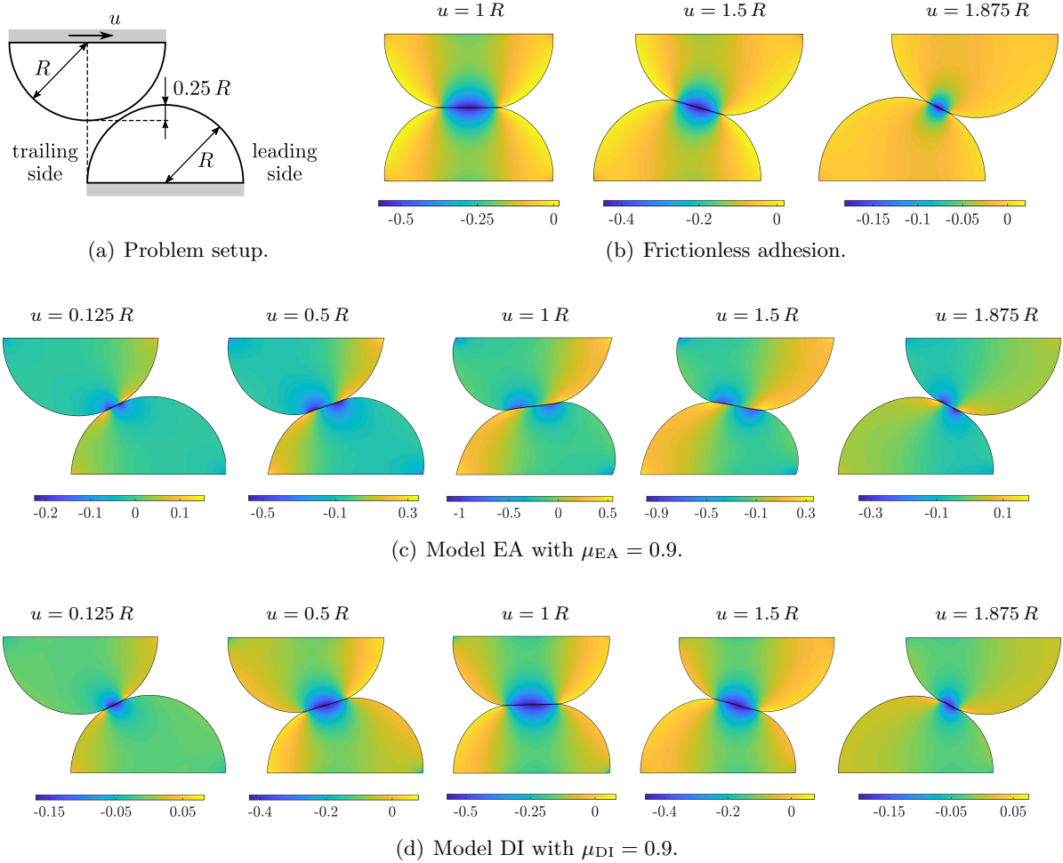
Figure 9 2D contact of two deformable cylinders: (a) Setup; (b) – (d) deformation during sliding for (b) frictionless adhesion or (c) & (d) models EA and DI with g_{cut} = g_{max} , respectively; note that the scaling of the colors (showing \text{tr } \boldsymbol{\sigma} / E ) is adjusted for each deformation state.
