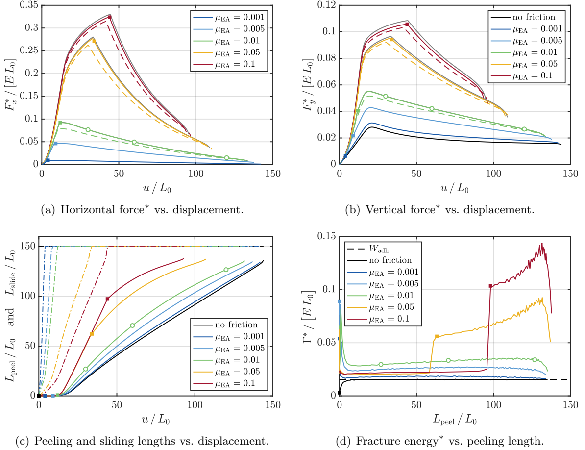
Figure 8 2D strip peeling: (a) & (b) Horizontal and vertical forces* (*: per out-of-plane width); solid colored lines: model EA with g_{\text{cut}} = g_{\text{max}} ; dashed colored lines: model EA with g_{\text{cut}} = (g_{\text{eq}} + g_{\text{max}})/2 ; solid gray lines: model DI with \mu_{\text{DI}} = \mu_{\text{EA}} and g_{\text{cut}} = g_{\text{max}} ; (c) nominal peeling length L_{\text{peel}} (solid) and nominal sliding length L_{\text{slide}} (dash-dotted); (d) fracture energy*; the white dots in Figs. (a) – (d) mark the configurations plotted in Fig. 6; the filled squares indicate the onset of full sliding rounded to next integer value of u .
