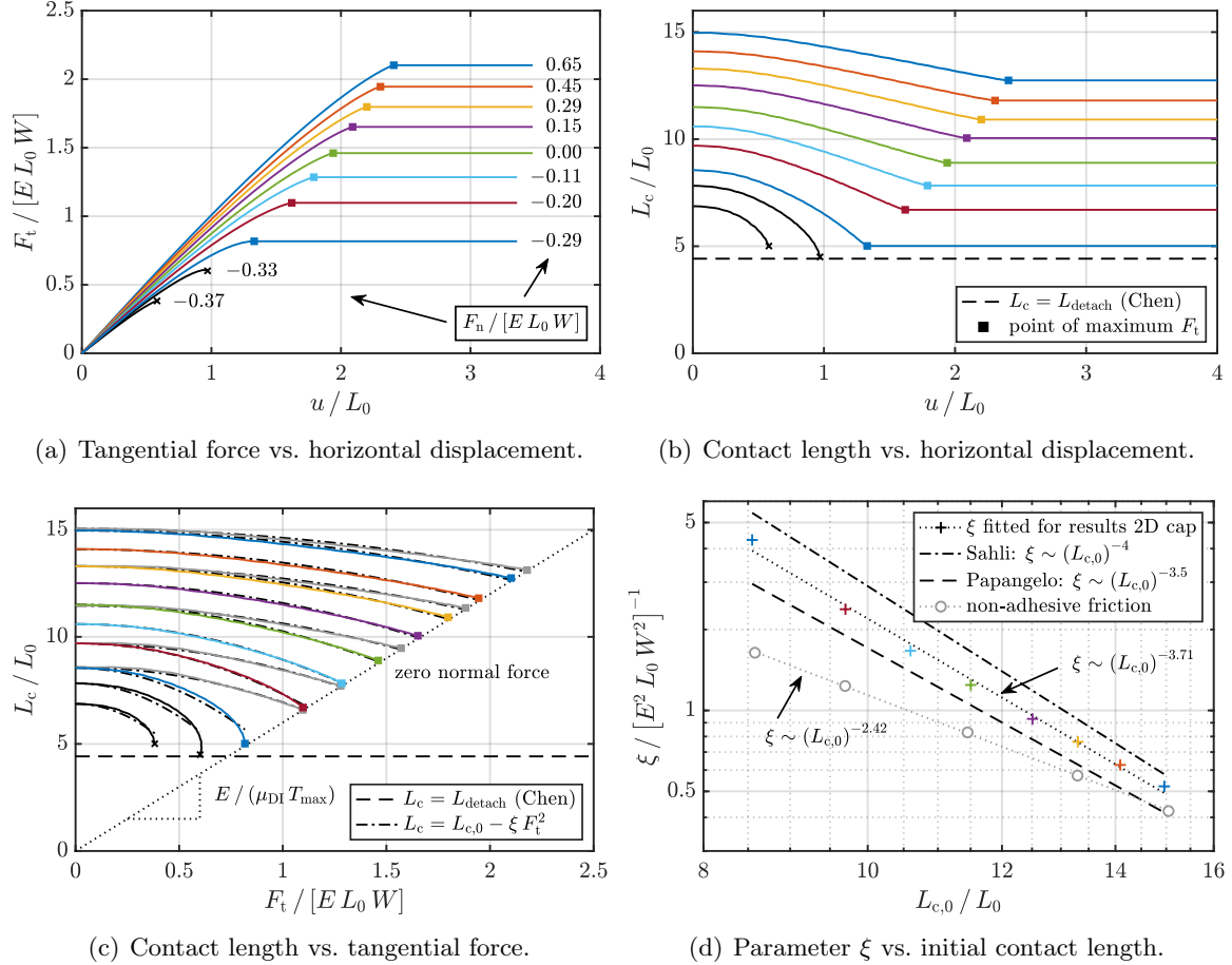
Figure 13 Adhesive friction of a 2D cap: (a) & (b) Tangential force and contact length, obtained for model DI ( g_{\text{cut}} = g_{\text{max}} , \mu_{\text{DI}} = 1 ) and different normal forces; the two solid black lines indicate contact vanishing under sufficient shear; (c) contact length in dependence of the tangential force; the five grey lines correspond to non-adhesive friction (Sect. 5.3); (d) parameter \xi from Eq. (37) fitted for all the cases from Fig. (c) with (non-vanishing) adhesive and non-adhesive contact.
