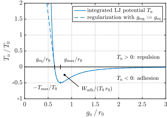
Figure 2 Normal contact traction in the model of Sauer and Wriggers (2009) for frictionless adhesion and repulsion as well as characteristic parameters; T_0 = A_{\text{H}} / (2\pi r_0^3) ; the blue dashed line shows a regularization of T_{\text{n}} based on linear extrapolation at g_{\text{n}} = g_{\text{eq}} ( Mergel et al., 2019 ).
