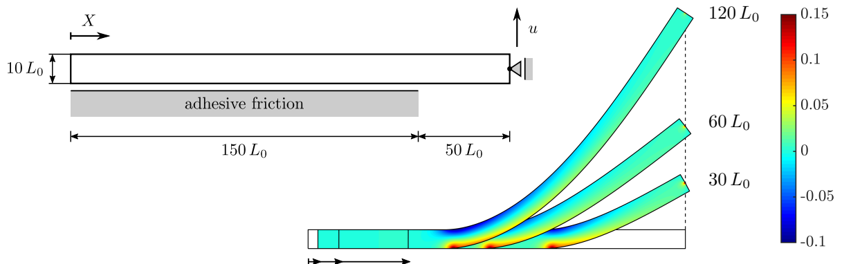
Figure 6 2D strip peeling: Setup (left) and three peeling states for model EA with g_{\text{cut}} = g_{\text{max}} and \mu_{\text{EA}} = 0.01 (right); the colors show the first invariant of the Cauchy stress, \text{tr } \boldsymbol{\sigma} , divided by E .
