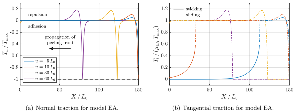
Figure 7 2D strip peeling: Traction at the contact area (in dependence of the horizontal position X normalized by L_0 ) for model EA with \mu_{\text{EA}} = 0.01 and g_{\text{cut}} = g_{\text{max}} ; the dash-dotted lines in Fig. (b) indicate sliding.
