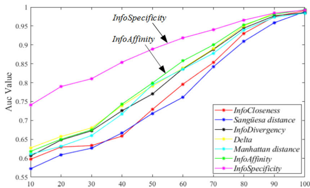
FIGURE 9. Comparison of the 7 similarity measures for Diabetes data base.
