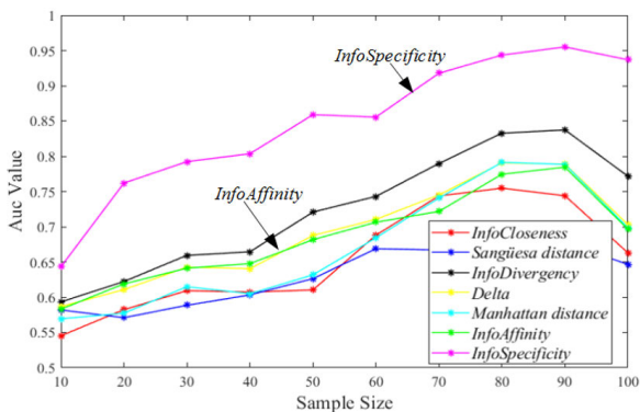
FIGURE 10. Comparison of the 7 similarity measures for Statlog data base.
