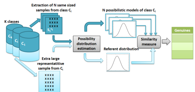
FIGURE 2. Gathering the geniuses: possibility distributions belonging to the same class.
