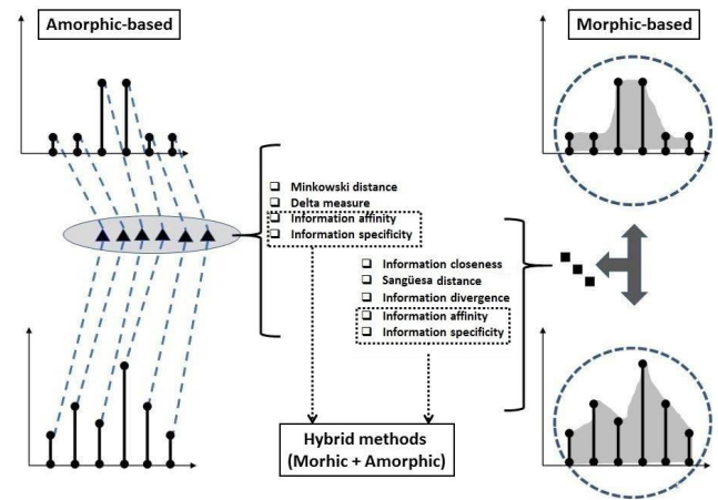
FIGURE 1. A typology of morphic and amorphous similarity measures.
