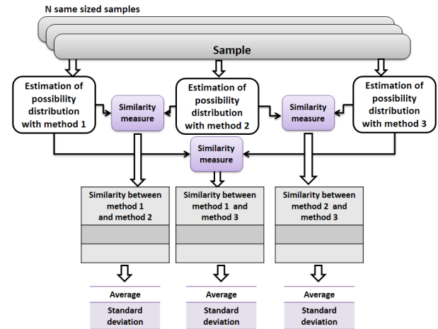
FIGURE 11. Similarity assessment of possibility distributions belonging to the same sample while estimated with different methods.
