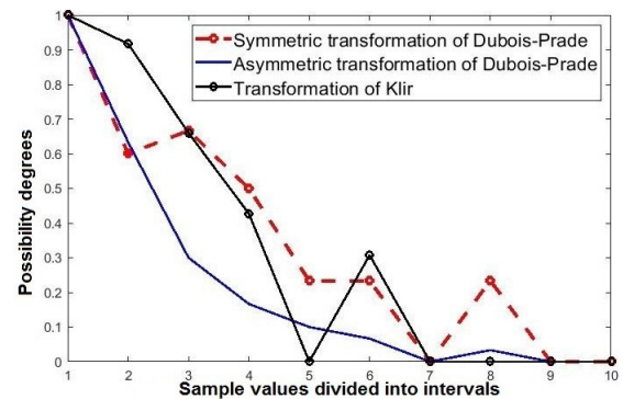
FIGURE 12. Application of different estimation methods on a sample of size=30 from Diabetes database.
