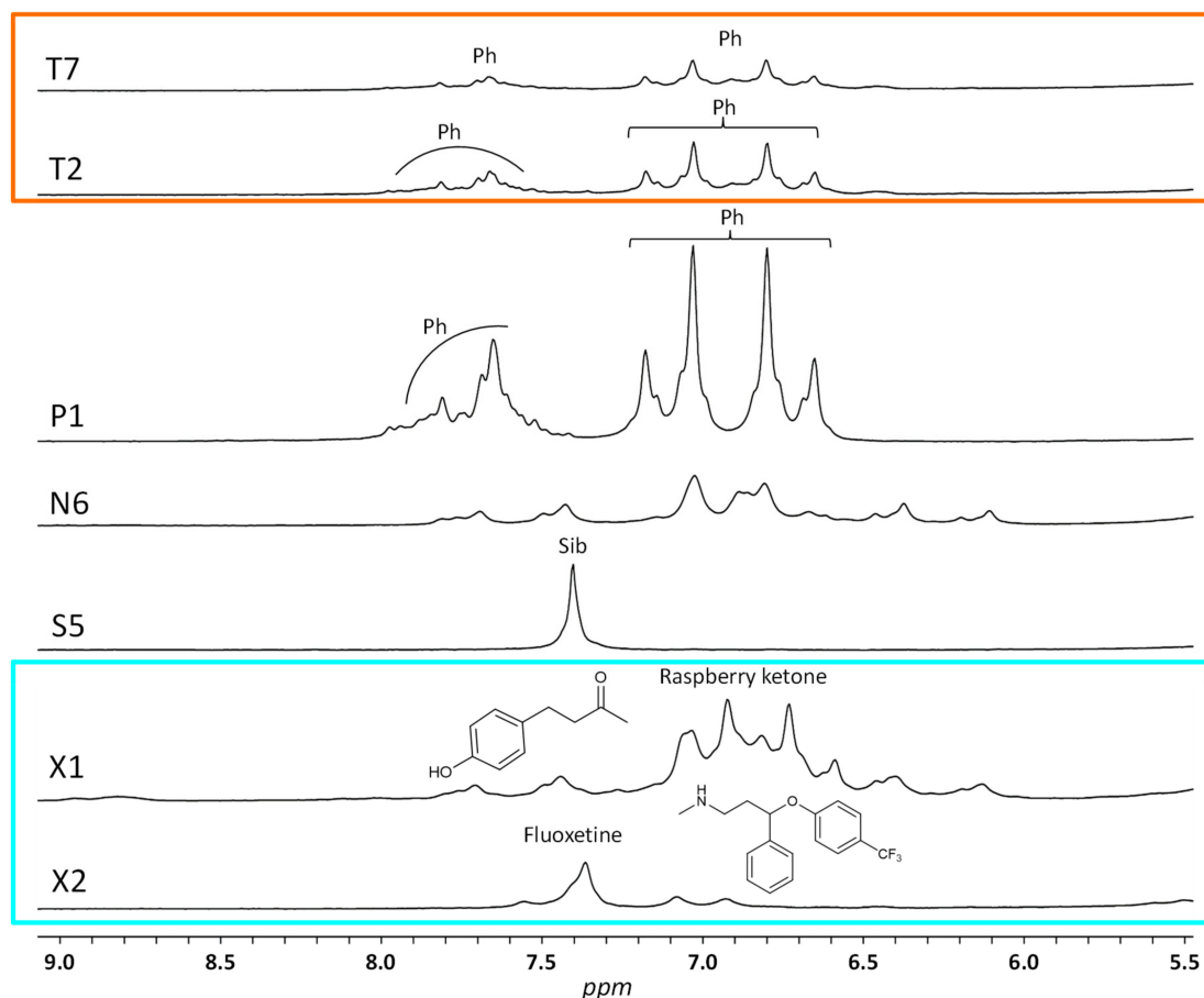
Figure 4. LF 1 H NMR spectra of some weight-loss dietary supplements recorded at 60 MHz. Ph: phenolphthalein; Sib: sibutramine.
