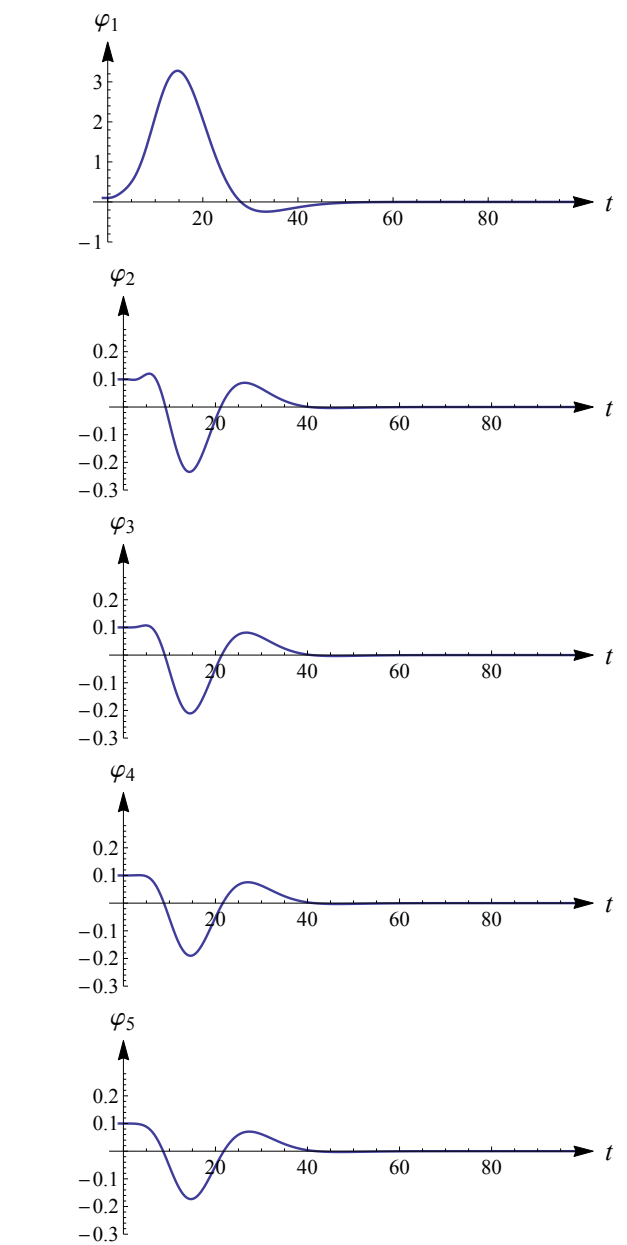
Fig. 2. Time-domain simulation for system (20) with 3g/l = 1 and \tau = 0.22 < \tau_0 .
