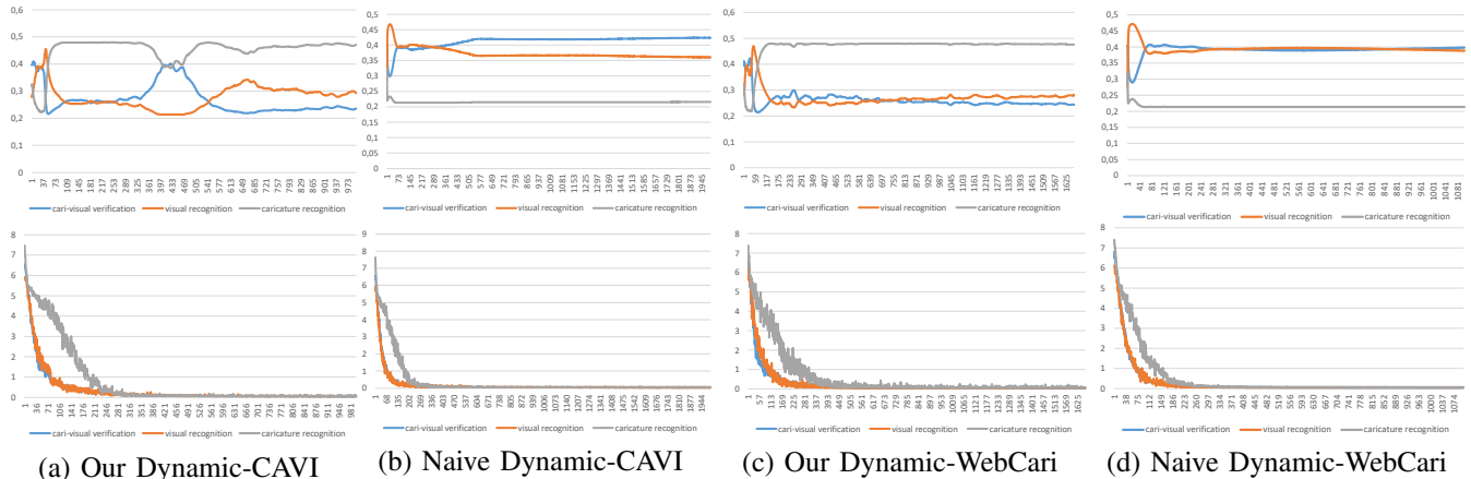
Figure 3. The evaluation of the proposed dynamic multi-task learning and the naive dynamic multi-task learning on the datasets CaVI and WebCaricature. The upper row shows the dynamic weights for both methods and the bottom row shows the corresponding losses. The grey curves denote the caricature recognition, the orange curves denote the visual recognition and the blue curves are the caricature-visual face verification. The vertical axis is the identification accuracy and the horizontal axis is the number of the training iterations.
