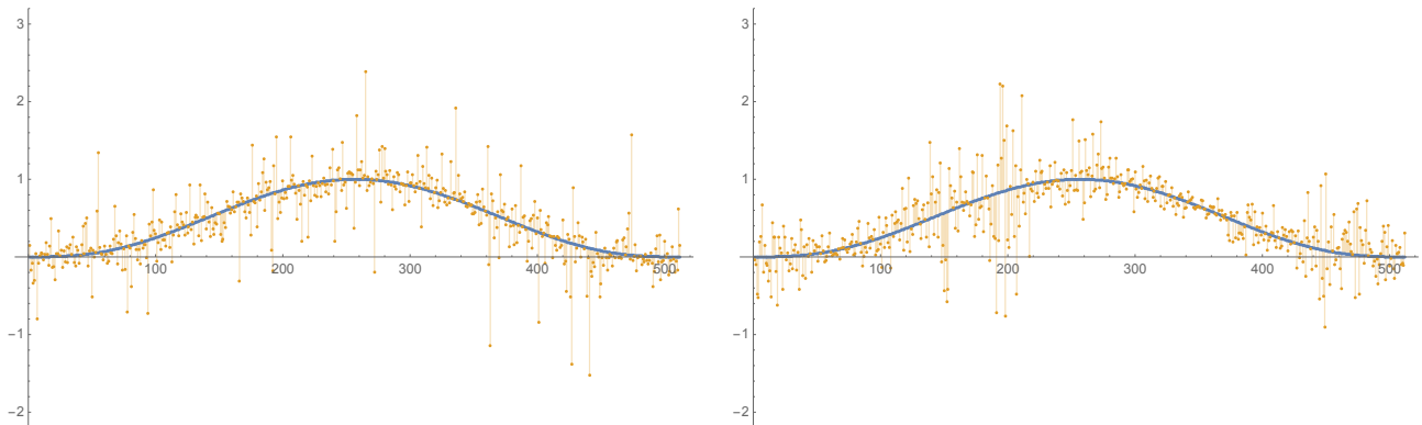
Figure 1 : n = 2^9 . Each of these 2 panels displays one data set Y and the “smooth” deterministic trend r(\cdot) when the noise is a log-normal SV sequence. In the 2 panels \tau = 0.75 , and they only differ by \gamma = 0.01 (left) and \gamma = 0.98 (right); see (17) for the definition of these two parameters.
