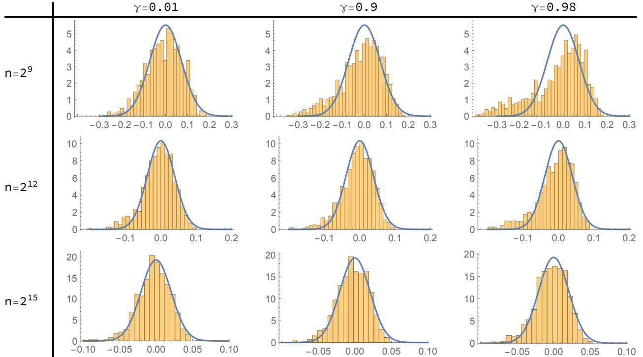
Figure 4 : \tau = 0.4 . These 9 panels only differ by n ( = 2^9 in the top row, 2^{12} (middle) and 2^{15} in the bottom row) and by \gamma varying in \{0.01, 0.9, 0.98\} . In each panel, the displayed normalized histogram is that of the 3000 replicates of \hat{h}_M - \hat{h}_n . The superposed blue curve is the normal distribution of \hat{h}_M - \hat{h}_n as predicted by the asymptotic theory.
