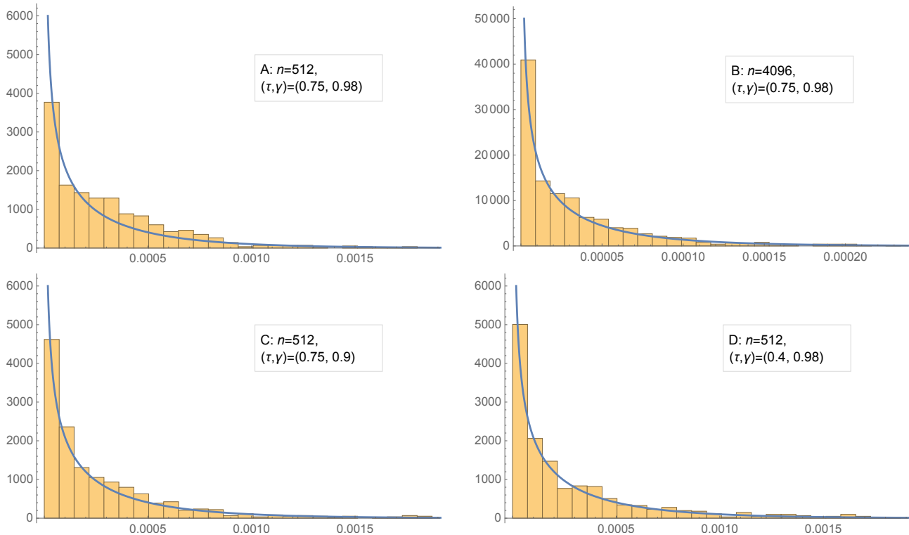
Figure 6 : Assessment of the simplified \frac{6}{5n}\sigma^2\mathcal{X}_2(1) approximation of the ASE-excess. In each panel, the displayed normalized histogram is that of the 3000 replicates of T_n(\hat{h}_M) - T_n(\hat{h}_n) . The superposed blue curve is the \frac{6}{5n}\sigma^2\mathcal{X}_2(1) density as suggested by the asymptotic theory. (A): n = 2^9 and (\tau, \gamma) = (0.75, 0.98) . (B): n = 2^{12} and (\tau, \gamma) = (0.75, 0.98) . (C): n = 2^9 and (\tau, \gamma) = (0.75, 0.9) . (D): n = 2^9 and (\tau, \gamma) = (0.4, 0.98) .
