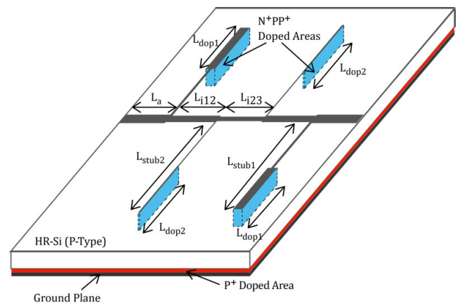
FIGURE 11. Design of the four-pole bandwidth switchable bandpass filter.
