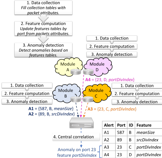
Figure 2: Architecture example. Local modules run at different points in the network and send alerts to the central correlation module. The controller will then be able to keep only distributed ones. Here it spots an anomaly on port 23 for feature portDivIndex , coming from two different places.
