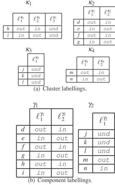
FIGURE 8 – Labellings computed using our algorithm.
