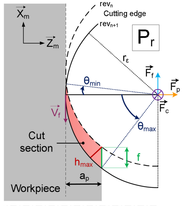
Fig. 1. Cutting edge engagement during face turning with a round cutting tool.
