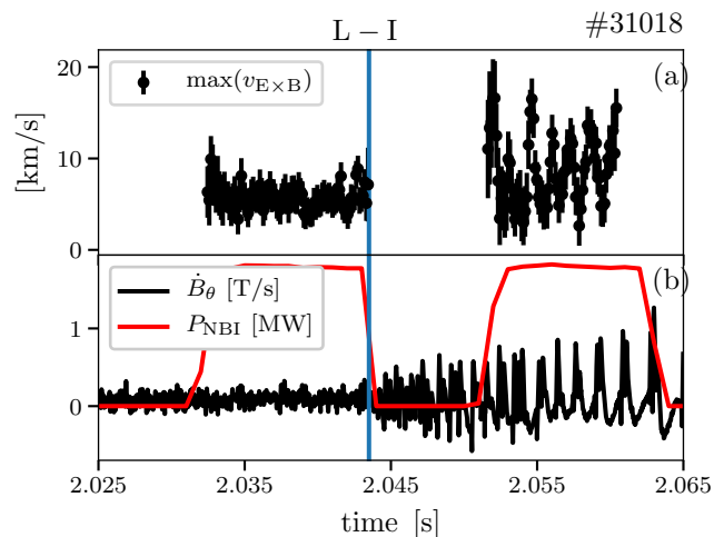
Figure 3: L-I transition triggered by an NBI blip. (a): \max v_{E \times B} , (b) NBI input power (red) and \dot{B}_\theta .
