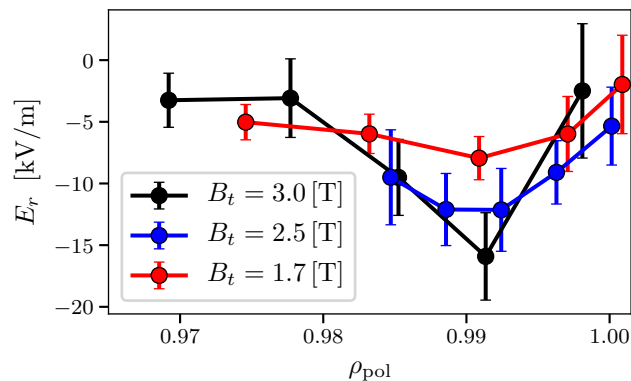
Figure 5: Edge E_r profiles at different magnetic fields before three single L-H transitions.
