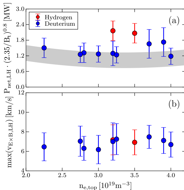
Figure 6: L-H power threshold normalized to 2.35 T (a) and maximum of v_{\mathbf{E} \times \mathbf{B}} as a function of the pedestal top density in hydrogen (red) and deuterium (blue) plasmas. The gray band in (a) indicates the measured P_{\text{thr}} for AUG as reported in [20].
