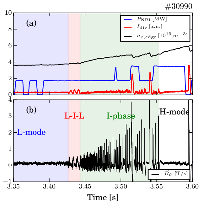
Figure 1: Evolution of a typical L-H transition at AUG considered in this work. (a): NBI power (blue), integrated edge electron density (black) and divertor shunt current (red), (b): Poloidal magnetic field fluctuation measured close to the secondary X-point.
