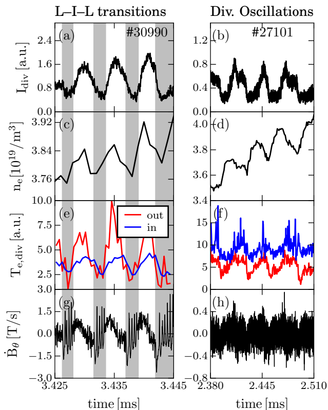
Figure 2: Comparison between L-I-L dithers (left-hand side) and divertor oscillations (right-hand side). (a)-(b) divertor shunt current, (c)-(d) edge electron density, (e)-(f) inner (blue) and outer (red) target temperatures, (g)-(h) poloidal magnetic fluctuations. The divertor oscillations are taken from a discharge published in [23].
