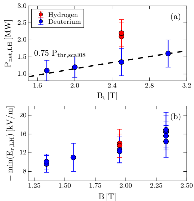
Figure 4: (a) L-H power threshold as a function of the toroidal magnetic field, (b) E_r minimum as a function of the local magnetic field at the measurement point. Discharges in hydrogen are shown in red and deuterium in blue. The dashed line in (a) indicates the power threshold scaling from [2] rescaled by 0.75 following the metal wall effect [20].
