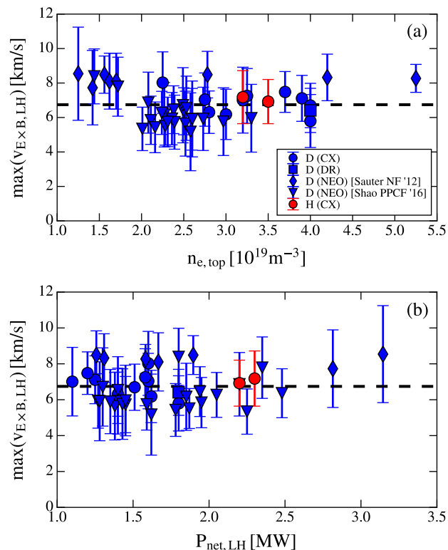
Figure 7: Maximum of v_{\mathbf{E} \times \mathbf{B}} as a function of the pedestal top electron density (a) and of the net input power (b). The figures compare data from CX, DR and from [9] and [18] (different symbols) while the different colors (red: hydrogen, blue: deuterium) indicate the different plasma isotope.
