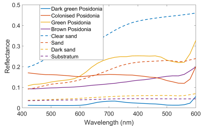
Figure 6. Various spectra representative of sand, Posidonia and substratum, collected in the studied area.
