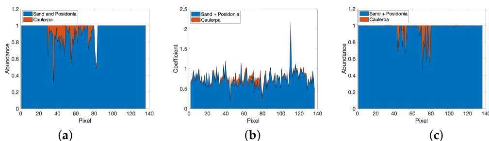
Figure 8. Part 2; (a) Abundances provided by the ground truth ( A_{CT} ); (b) LS coefficients ( C_{est} ); (c) Abundances obtained using WADJUM ( A_{est} ).
