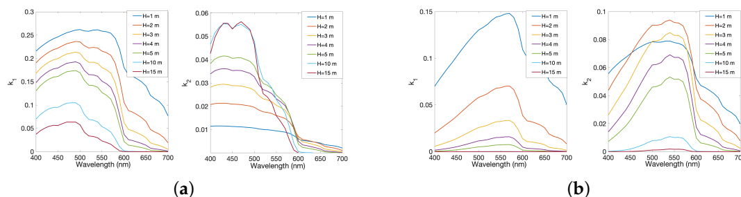
Figure 2. Direct and diffuse water column attenuation (respectively \mathbf{k}_1 and \mathbf{k}_2 vectors); (a) Clear water ( Chl = 0.03 \text{ mg}\cdot\text{m}^{-3} , SM = 0.01 \text{ mg}\cdot\text{L}^{-1} , CDOM = 0.01 \text{ m}^{-1} ); (b) Moderately turbid water ( Chl = 1 \text{ mg}\cdot\text{m}^{-3} , SM = 1 \text{ mg}\cdot\text{L}^{-1} , CDOM = 0.1 \text{ m}^{-1} ).
