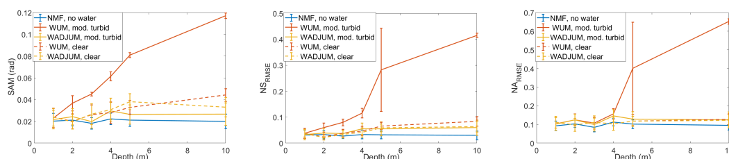
Figure 3. Spectral angle mapper, mean normalized RMSE errors on estimated spectra and estimated abundances using unmixing methods for various cases: when no water column is present ( NMF , no water), when the water column is present but the adjacency effects induced by the seabed and the water column are ignored ( WUM ), and when the water column and the adjacency effects are accounted for ( WADJUM ), for clear and moderately turbid water conditions. \mathbf{K}_1 , \mathbf{K}_2 and \delta are known.
