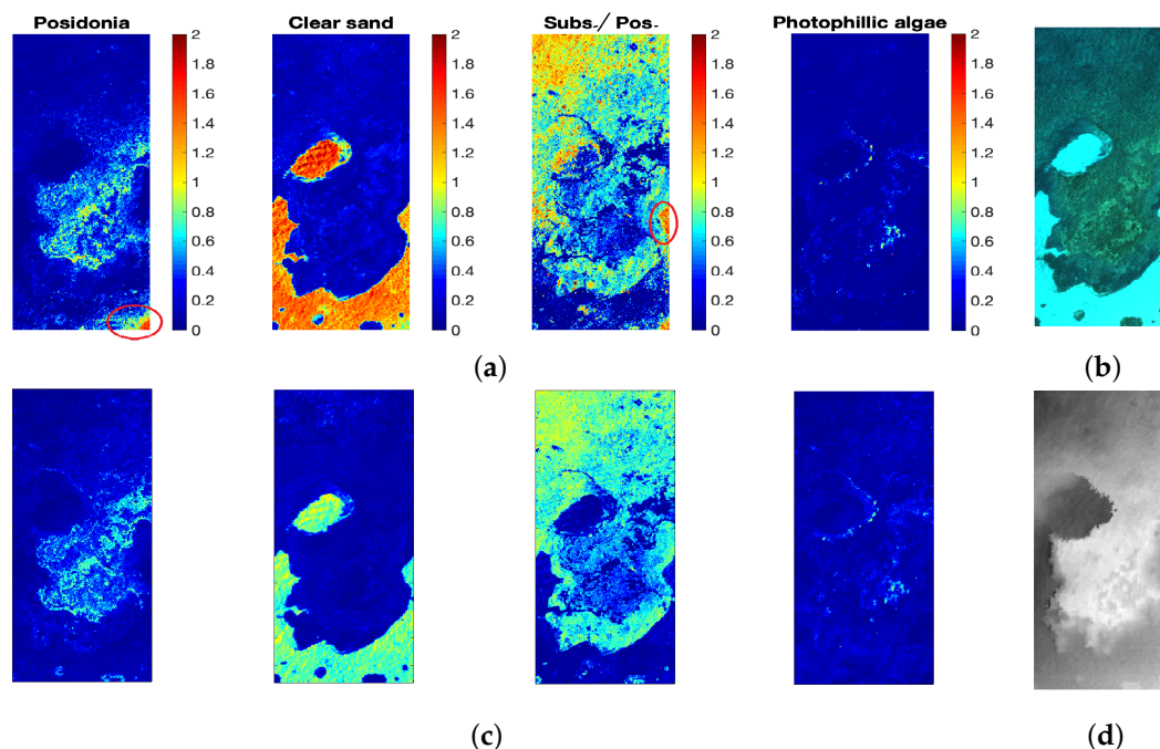
Figure 9. (a) Coefficients ( \mathbf{C}_{est} ), estimated using LS inversion; (b) Airborne reflectance data of the Porquerolles Island, taken using the Hypspec hyperspectral sensor (sub-surface correction); (c) Abundances ( \mathbf{A}_{est} , estimated using WADJUM ); (d) Bathymetry provided by the Litto3D database. The depth is between 1.8 m (white) and 6.1 m (black).
