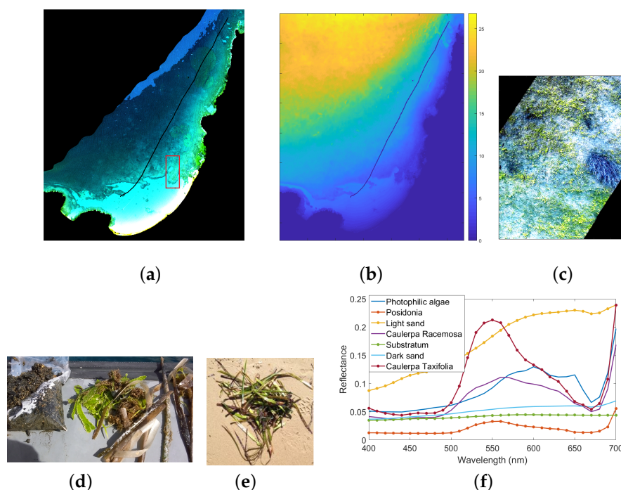
Figure 5. (a) Colored composition of the airborne reflectance data of the Porquerolles Island, acquired using the Hypspec hyperspectral sensor (with sub-surface and sun glint correction), with the trace of the ROV transect (black), and local study zone (red rectangle); (b) Bathymetry provided by the Litto3D data; (c) Color image of the seabed given by the Ifremer ROV, showing clear and dark sand, brown Posidonia , and Caulerpa (green); (d) Dark substratum, Caulerpa taxifolia and brown colonized Posidonia ; (e) Green Posidonia on clear sand; (f) Spectral library collected in the coastal zone of Porquerolles Island, used for simulations (the endmembers used for the seabed generation are marked with a dot).
