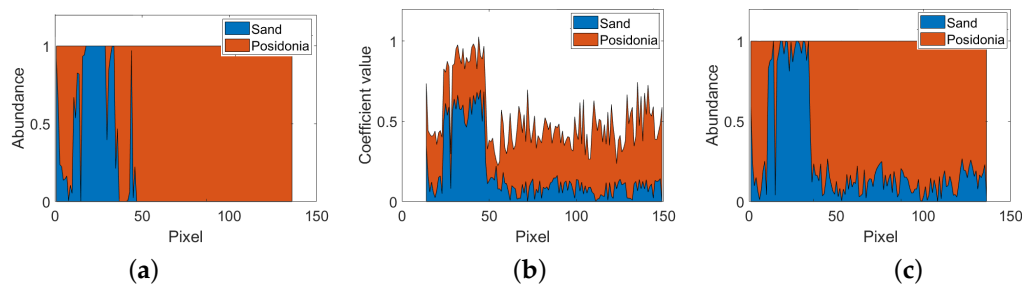
Figure 7. Part 1; (a) Abundances provided by the ground truth ( A_{CT} ); (b) LS coefficients ( C_{est} ); (c) Abundances obtained using WADJUM ( A_{est} ).
