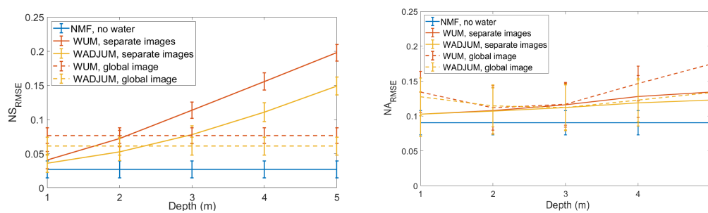
Figure 4. Normalized RMSE for endmember spectra ( NS_{RMSE} ) and abundances ( NA_{RMSE} ), for five separate constant seabed depth areas (plain lines), and for the entire image composed of all five areas (dashed lines), obtained using biased values of K_1 , K_2 and \delta induced by a lack of knowledge for the water quality, in the case of moderately turbid water and z = [1, 2, 3, 4, 5] m.
