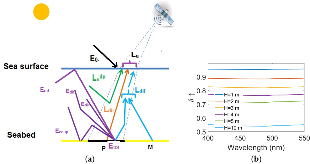
Figure 1. (a) Various components of the light that contributes to the sub-surface radiance (from [45]). The reader is referred to Table 1 for the definition of the notations used in the Figure. (b) Environment vector \delta \uparrow , which represents the weight of the target pixel contributing to the diffuse radiance, for a target radius of 0.5 m, for various seabed depths ranging from 1 m to 10 m, and moderately turbid water conditions, corresponding to a chlorophyll-a concentration Chl = 1 \text{ mg m}^{-3} , a suspended matter concentration SM = 1 \text{ mg L}^{-1} , and a color dissolved organic matter concentration CDOM = 0.1 \text{ m}^{-1} .
