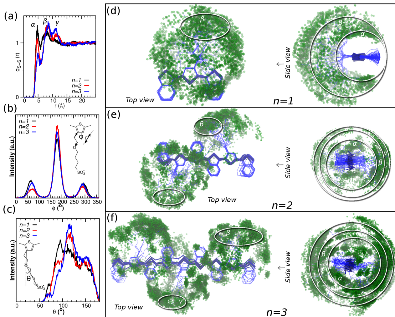
Figure 4. (a) Radial distribution function g_{S-S}(r) for the distance between S from \text{SO}_3 and S from the thiophene ring for different chain lengths, n . (b) Probability distribution function, P(\phi) and definition of dihedral angle between neighbouring atoms in the aliphatic chain, \phi . (c) Probability distribution function, P(\theta) and definition of the angles between aryl-C, ether-O and sulfonate-S, \theta . (d)-(f) Folding of sulfonate groups (green spheres) on the plane of ETE-S chains (blue) is visualized by plotting them with their thiophene rings aligned; chain lengths n = 1, 2, 3 respectively; water content is 29% w/w. No hydrogen atoms are showed. Circles and ellipses indicate the corresponding location of the \text{SO}_3 groups given by peaks \alpha, \beta, \gamma in the distribution function g_{S-S}(r) in (a).
