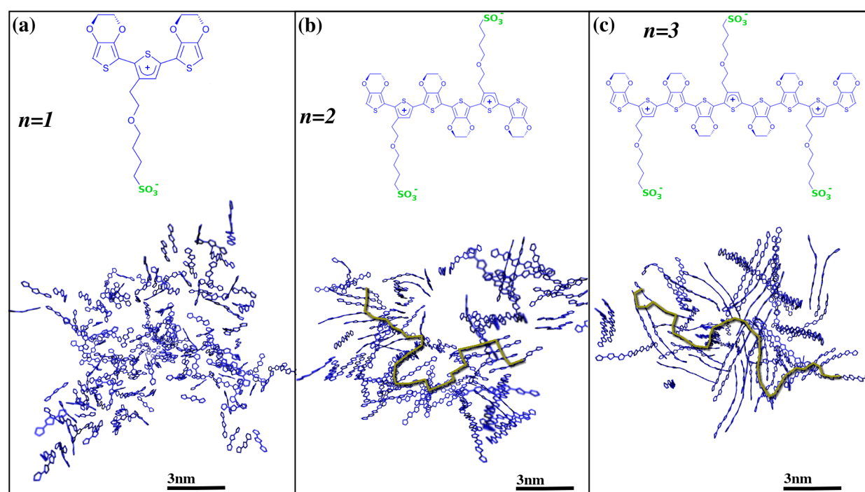
Figure 1. (a)-(c) Upper. Schematic representation of self-doped oligomer ETE-S chains for n=1, 2 and 3 . Positive charges in the backbone +ne is compensated by negative charges -e in each sulfonate group. Below. Snapshots of the aqueous ETE-S solution for different chain length n=1, 2 and 3 ; water content is 29.3% w.t. (Only thiophene rings from ETE-S chains are showed for clarity; water is not displayed). Representative percolative paths for charge carriers between ETE-S chains are indicated in green. (Percolative paths are defined as the paths that connect neighboring thiophene rings on the same ETE-S chain or on neighboring \pi - \pi stacked chains).
