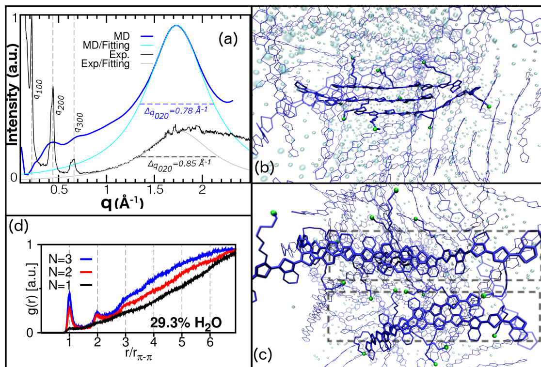
Figure 2. (a) Experimental GIWAXS pattern of the cast oligomer film cast and calculated X-ray diffraction pattern on the simulated ETE-S, n=3 at a water content of 29.3 % w.t. (d) Radial distribution function between oligomer chains with n=1,2 and 3. (b)-(c) The production snapshot with n=3 from side and top view, respectively. ETE-S chains are represented in blue, sulfonate groups are illustrated by the S atom in green and water molecules by O atoms in light blue. H atoms are not shown. Rectangular boxes in (c) show two neighboring crystallites outlining the formation of lamellar structure.
