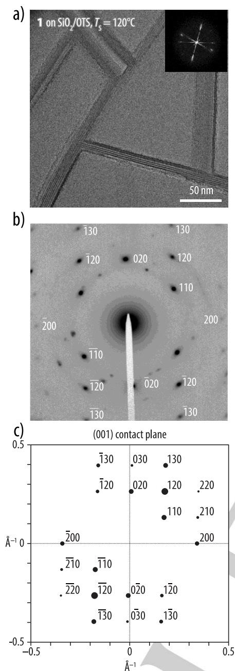
Figure 4. a) High-resolution transmission electron microscopy (HR-TEM) images of films of 1 deposited onto SiO 2 /OTS at T S = 120°C; the inset shows the fast Fourier transformation (FFT) from the HR-TEM images, revealing a periodicity of approximately 26 Å for the needle-like domains. b, c) Representative selected-area electron diffraction (SAED) map of the films of 1 showing good agreement with the calculated diffraction map from the single crystal of 1 (see Supplementary Figure S9, Supplementary Table S1), indicating the coexistence of a (001) and (00-1) contact plane.
