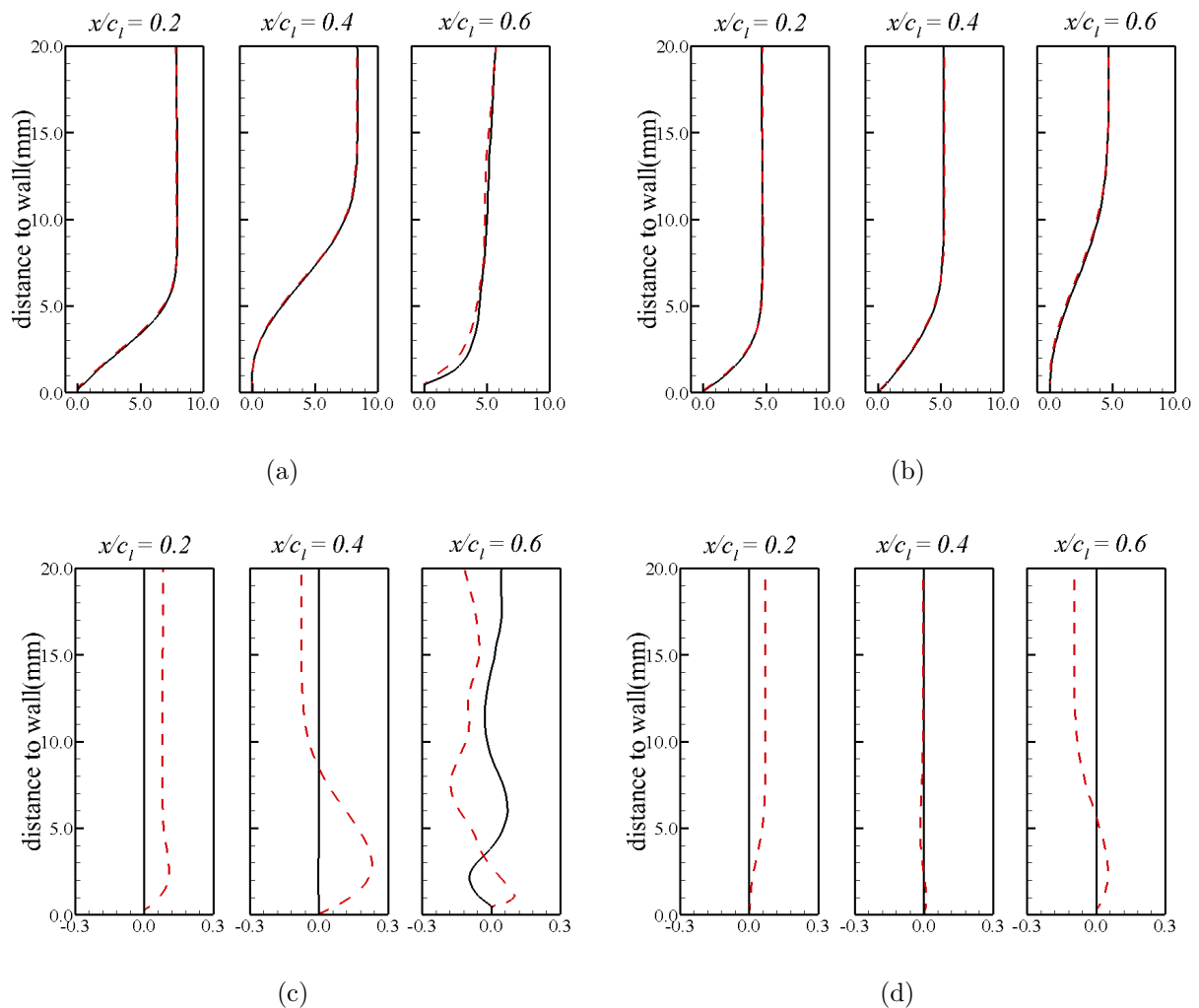
Figure 5: Velocity profile --- 3D rotating blade — Airfoil (a) Streamwise velocity, Suction side (b) Streamwise velocity, Pressure side (c) Cross-flow velocity, Suction side (d) Cross-flow velocity, Pressure side
