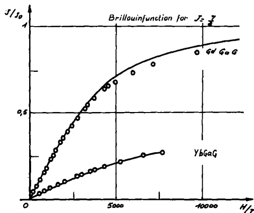
Fig. 9. Variations of the relative magnetisations versus H/T for Gd Ga G and Yb Ga G and the corresponding Brillouin function.
