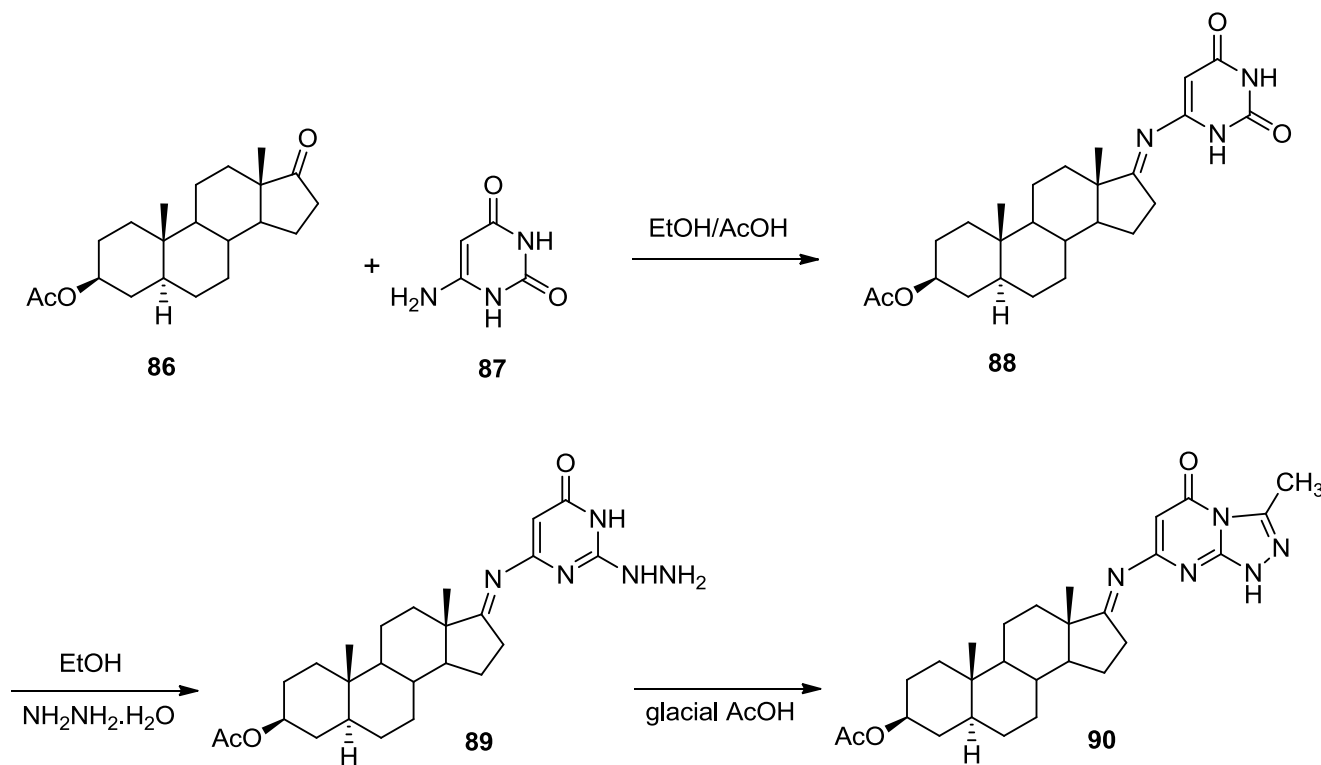
14 15 16 Scheme 19. Synthesis of compounds 88 , 89 and 90 .
