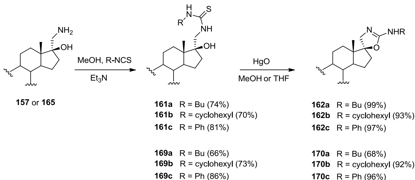
Scheme 35. Synthesis of 2-aminoxazolines 162 , 170 from trans -androsterone and estrone.
