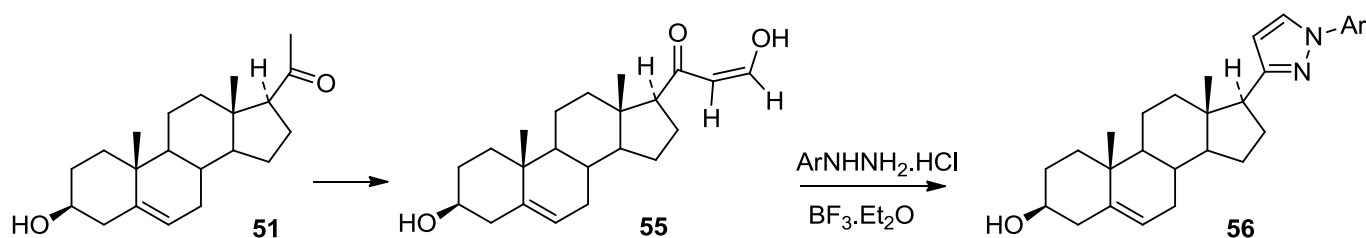
12 13 14 Scheme 15. Synthesis of D-ring substituted pyrazolyl-pregnenolones. 15
