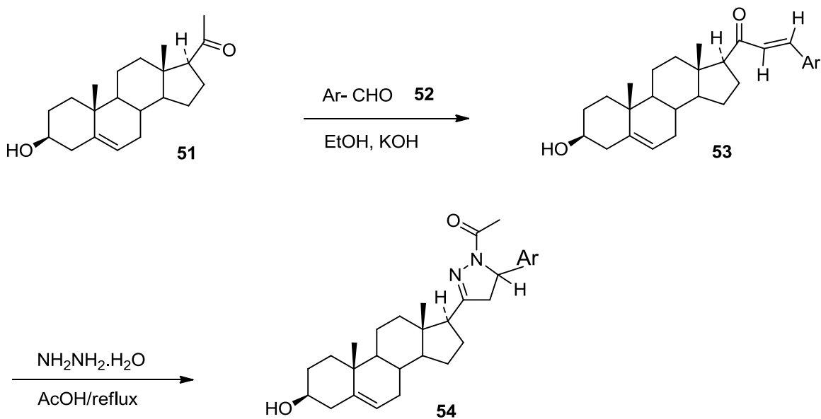
4 5 Scheme 14. Synthesis of D-ring substituted pyrazolinyl-pregnenolones. 6
