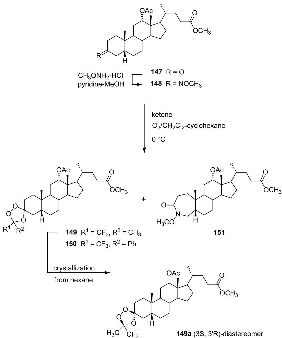
8 9 10 Scheme 32. Preparation of the ozonide 149a .
