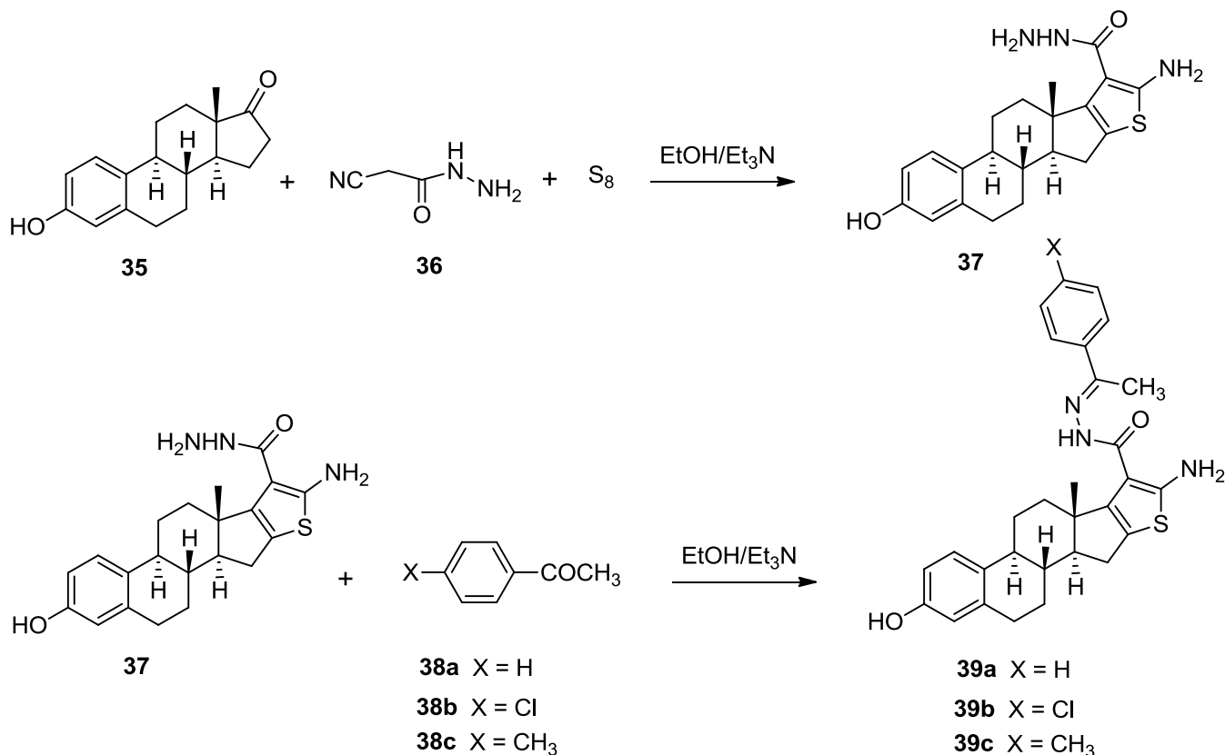
9 10 11 Scheme 11. Synthesis of compounds 37 and 39a-c . 12
