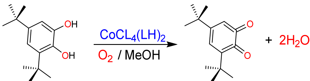
Scheme 2. Catalytic oxidation of 3,5-DtBC to 3,5-DtBQ.
