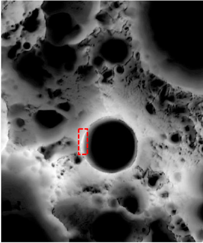
Fig. 1. Multi-temporal illumination map of the lunar South Pole. The Shackleton crater (19 km diameter) is in the center. The South Pole is located approximately at 9 o'clock on its rim (highlighted red). Mapped area extends from 88°S to 90°S (NASA/GSFC, 2010).
