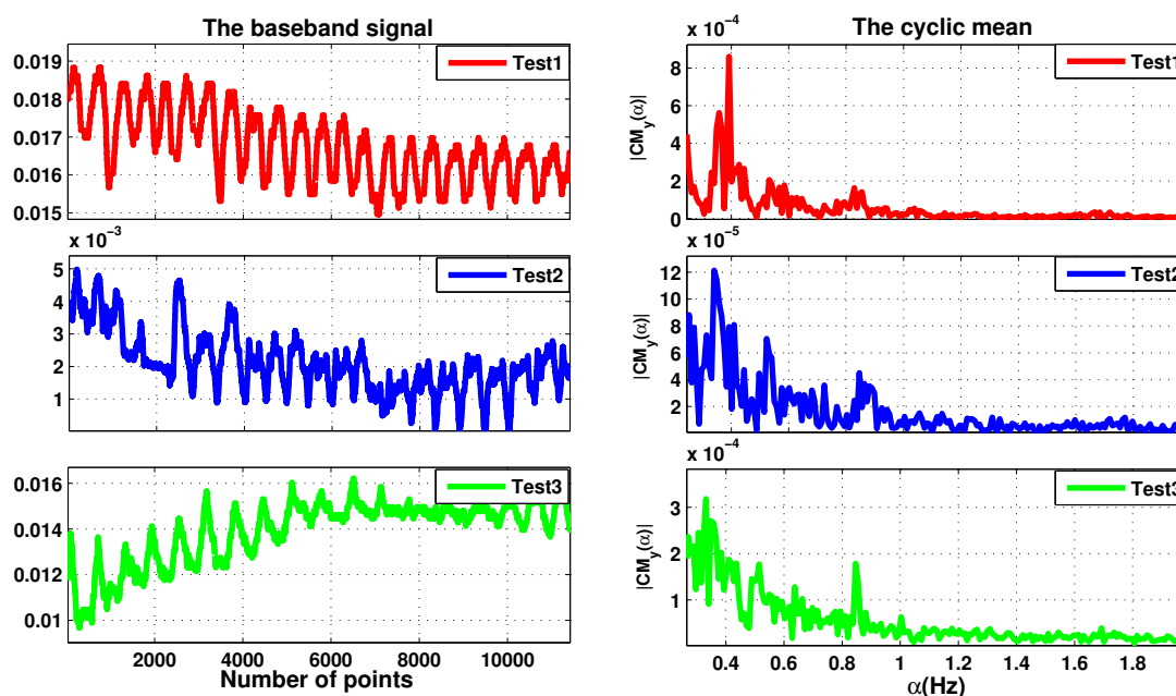
Figure 14. The baseband signal measured in different positions of the person-under-test and their cyclic means.
