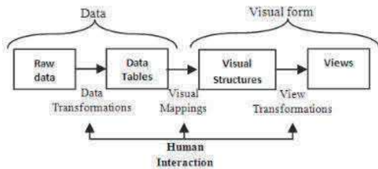
Fig. 5. Interactive Mechanism [31]
