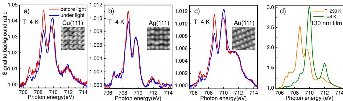
Figure 1: 4 K X-ray absorption spectra of the \text{Fe}^{\text{II}} L_3 edge before and after illumination of the sample with a blue light (405 nm) for 20 minutes for : a) 0.4\pm 0.1 ML of (1) on Cu(111). b) 0.5\pm 0.1 ML of (1) on Ag(111). Average over 11 spectra before light and 10 spectra under light in steady state conditions. c) 0.5\pm 0.1 ML of (1) on Au(111). Average over 6 spectra before light and 13 spectra under light in steady state conditions. A linear background has been removed and the spectra have been normalized to the background value at 708.7 eV. The jump at the L_3 edge can therefore be read as a percentage of the background signal. In inset, 5\times 5 \text{ nm}^2 STM images recorded at tunneling conditions : U=-1.3 \text{ V} , I=50 \text{ pA} on Cu(111), U=-1.5 \text{ V} , I=10 \text{ pA} on Ag(111) and U=-1.5 \text{ V} , I=20 \text{ pA} on Au(111). d) Reference spectra recorded at 4 K and 290 K on a 130 nm thick film of (1) on a \text{SiO}_2 substrate.
