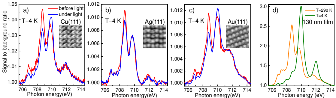
Figure 1: 4 K X-ray absorption spectra of the \text{Fe}^{\text{II}} L_3 edge before and after illumination of the sample with a blue light (405 nm) for 20 minutes for : a) 0.4\pm 0.1 ML of (1) on Cu(111). b) 0.5\pm 0.1 ML of (1) on Ag(111). Average over 11 spectra before light and 10 spectra under light in steady state conditions. c) 0.5\pm 0.1 ML of (1) on Au(111). Average over 6 spectra before light and 13 spectra under light in steady state conditions. A linear background has been removed and the spectra have been normalized to the background value at 708.7 eV. The jump at the L_3 edge can therefore be read as a percentage of the background signal. In inset, 5\times 5 \text{ nm}^2 STM images recorded at tunneling conditions : U=-1.3 \text{ V} , I=50 \text{ pA} on Cu(111), U=-1.5 \text{ V} , I=10 \text{ pA} on Ag(111) and U=-1.5 \text{ V} , I=20 \text{ pA} on Au(111). d) Reference spectra recorded at 4 K and 290 K on a 130 nm thick film of (1) on a \text{SiO}_2 substrate.
