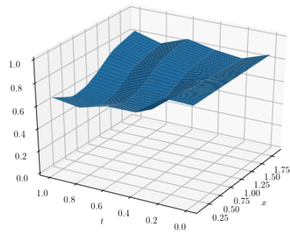
Figure 13: \bar{a}^{\bar{L}, \hat{\theta}^{L,*}}(t, x)
