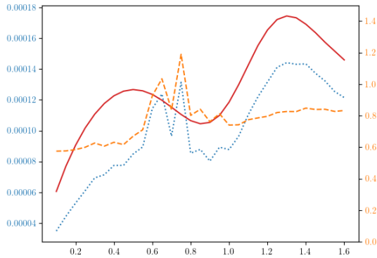
Figure 62: Standard Deviation vs x_0 for Full Method
