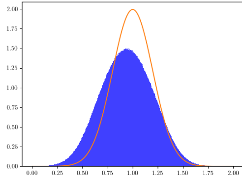
Figure 27: \bar{X}_T Distribution Under \mathbb{Q}^{\hat{\theta}^*}
