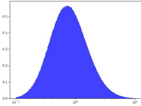
Figure 10: \bar{Z}_T^{\hat{\theta}^*} Distribution Under \bar{Q}^{\bar{L}, \hat{\theta}^{L,*}}
