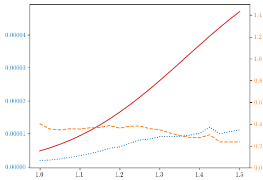
Figure 6: Standard Deviation vs x_0 for Full Method
