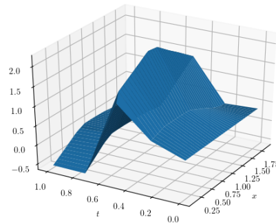
Figure 65: \tilde{a}^{\theta}(t, x)
