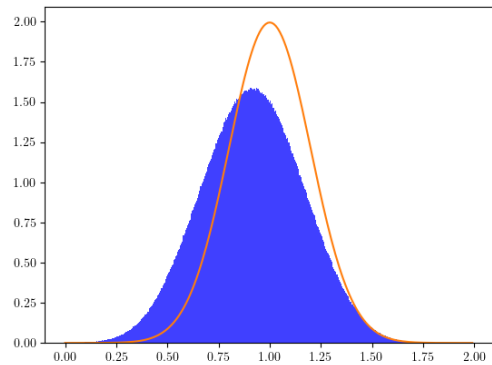
Figure 29: \bar{X}_T Distribution Under \mathbb{Q}^{L, \hat{\theta}^{L,*}}
