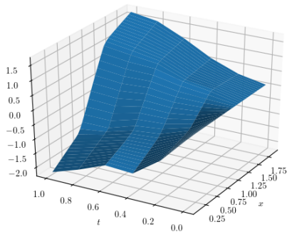
Figure 30: \tilde{a}^{\hat{\theta}^*}(t, x)
