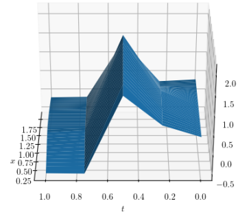
Figure 67: \tilde{a}^\theta(t, x)
