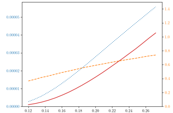
Figure 75: Standard Deviation vs \sigma , Adaptive vs MC - Bachelier Diffusion - Multi Coupons AutoCall
