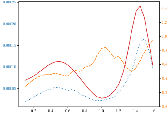
Figure 34: Standard Deviation vs x_0 for Full Method
