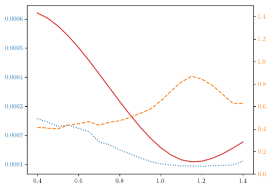
Figure 48: Standard Deviation vs x_0 for Full Method
