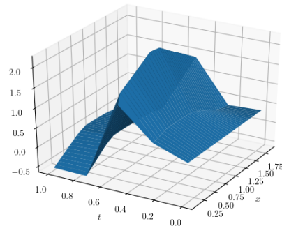
Figure 65: \tilde{a}^{\theta}(t, x)
