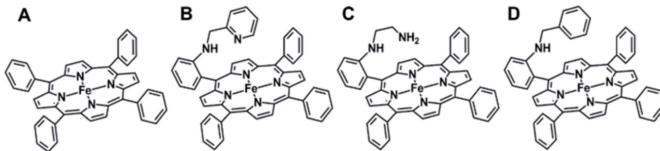
Fig. 2 Molecular structures of iron–porphyrin complexes used in this study: (A) \text{Fe}^{\text{III}}\text{TTP} , (B) \text{Fe}^{\text{III}}\text{L2} , (C) \text{Fe}^{\text{III}}\text{L3} and (D) \text{Fe}^{\text{III}}\text{MPh} .
