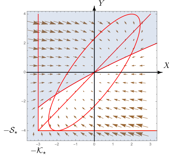
FIGURE 1. In (X, Y) coordinates, arrows represent the vector field which corresponds to (6.13), i.e., (\Lambda Y - 4X, -BY) . The line \Lambda Y - 4X = 0 determines the sign of X' . The ellipse defined by (6.16) is also represented. White areas are the regions such that (6.11) holds: the upper limit is Y = \psi(X) . Here we have d = 3 , m = m_1 = 2/3 , \Lambda = 2d(1-m)/m = 3 and B = 2d(m - m_c) = 2\alpha and scales are in units of \mathcal{M} . The qualitative properties are independent of the dimension d \geq 3 and of the exponent m \in [m_1, 1) .
