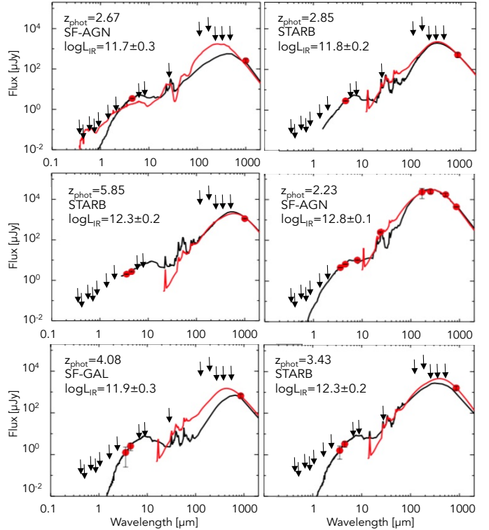
Fig. 10. Observed SEDs for HST+near-IR-dark galaxies, with their tentative best fitting templates (black for the broad-band SED and red for the far-IR SED, as in Fig. 6) and photometric redshifts found with LE PHARE. For all but one source, the fits are based only on the IRAC and ALMA data points, combined with the 3\sigma UV, optical, near- and far-IR 3\sigma upper limits.
