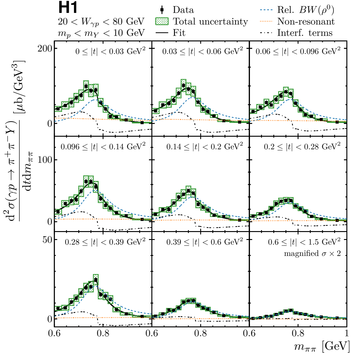
Figure 13: Proton-dissociative ( m_p < m_Y < 10 GeV) double-differential \pi^+ \pi^- photoproduction cross sections d^2 \sigma(\gamma p \rightarrow \pi^+ \pi^- Y)/dm_{\pi\pi} dt in bins of t and as functions of m_{\pi\pi} . The model that is fitted to the data as described in the text and its components are also shown.
