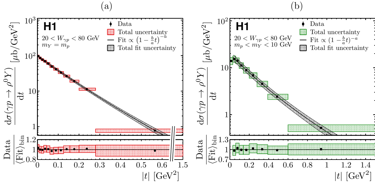
Figure 14: Elastic ( m_Y=m_p ) (a) and proton-dissociative ( m_p < m_Y < 10 \text{ GeV} ) (b) differential \rho^0 meson photoproduction cross sections d\sigma(\gamma p \rightarrow \rho^0 Y)/dt as functions of t . The distributions are parametrised with fits as described in the text, and the fitted curves are also shown. In the ratio panels, the data are compared to the bin-averaged fit function values as they entered in the \chi^2 calculation for the fit. The depicted bin centres are evaluated using the fit functions as described in the text.
