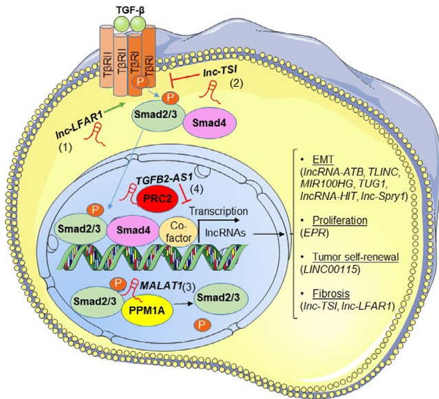
FIGURE 2 TGF-β signaling regulates lncRNA expression and mechanisms of TGF-β signaling control by lncRNAs. TGF-β signals through Smad2/3/4 proteins to regulate the expression of lncRNAs, acting as effector molecules that mediate the physiological responses of the signaling pathway (listed on the right hand-side). lncRNAs target TGF-β signaling at different stages of the pathway. At the level of Smad2/3 activation by TGFβRI, lnc-LFAR1 (1) enhances the association of Smad2/3 with TGFβRI, leading to increased activation of the pathway. lnc-TSI (2) blocks the interaction of Smad3 with TGFβRI, attenuating the pathway. In the nucleus, MALAT1 (3) shifts the Smad2/3 levels toward the non-phosphorylated state, by promoting the association of the phosphatase PPM1A to Smads and inhibiting TGF-β-mediated responses. TGFβ2-AS1 (4) epigenetically silences TGF-β-target genes by recruiting the PRC2 repressive complex to their promoters
