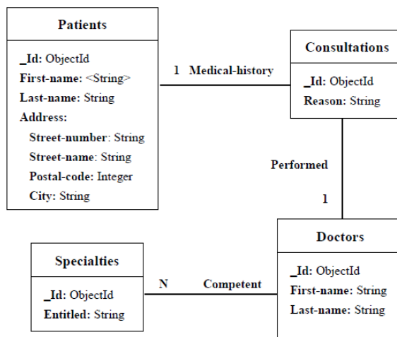
Figure 1: Excerpt from the physical model of data.
