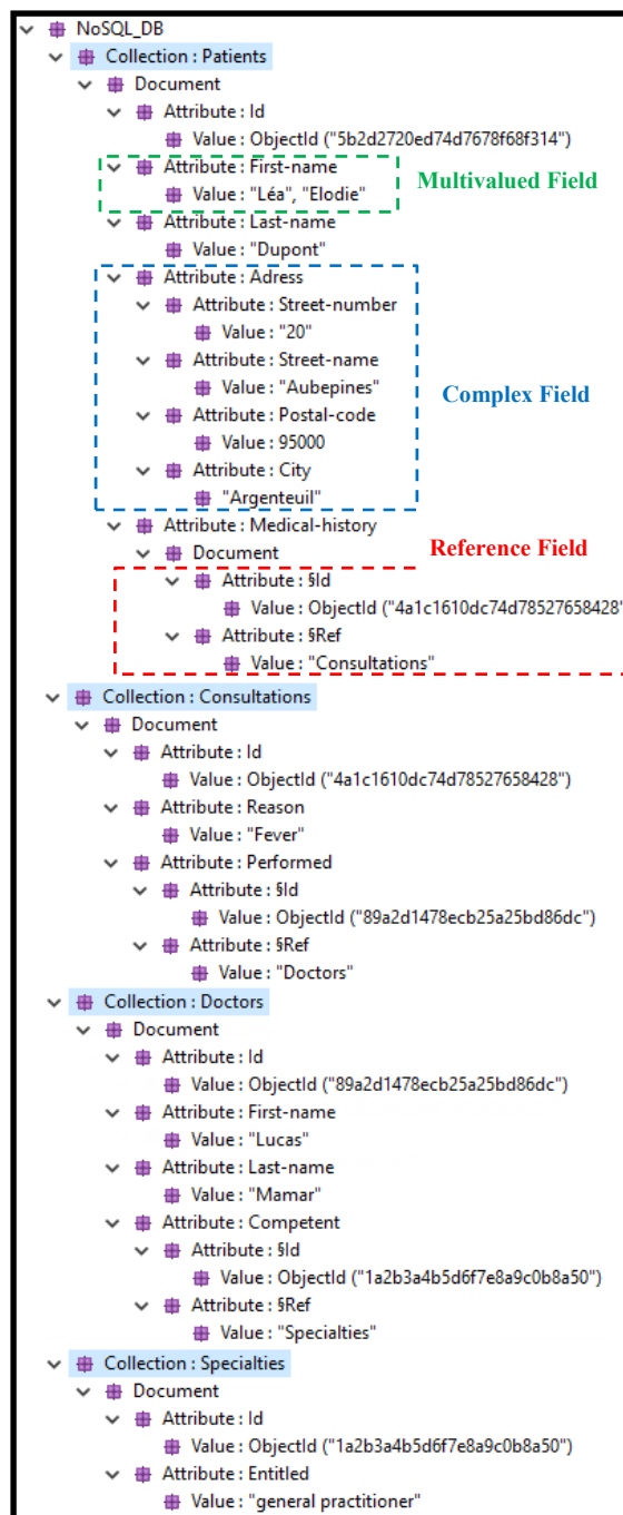
Figure 5: Source Model.
