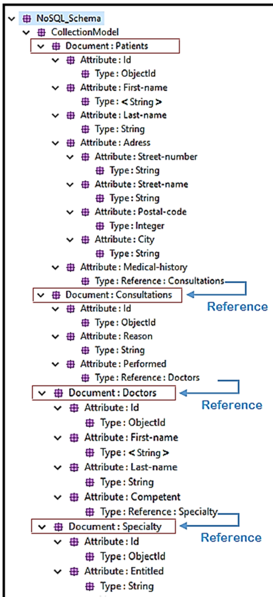
Figure 6: Target Model.
