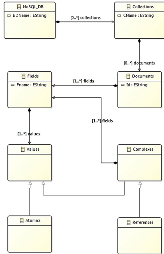
Figure 3: Source Metamodel.
