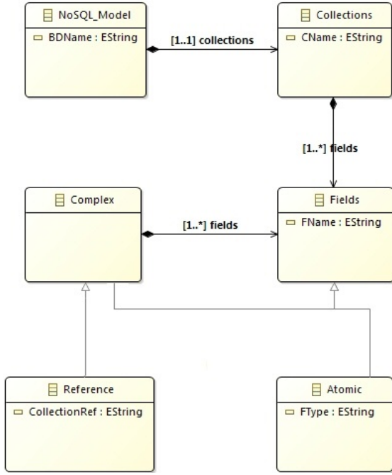
Figure 4: Target Metamodel.
