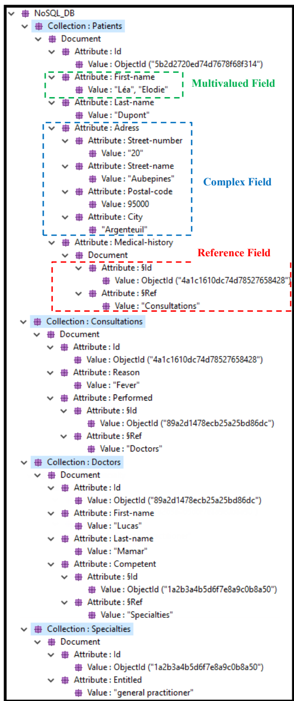
Figure 5: Source Model.
