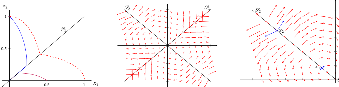
(a) The blue line shows a trajectory starting from (0,1) , the red line a trajectory starting from (0.5,0) and the red dashed line indicates a level set of V(x) .
