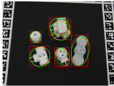
Fig. 2. Ground truth ellipses obtained by projecting the ellipsoids with the ground truth camera matrix are in green, whereas bbox ellipses are in red.
