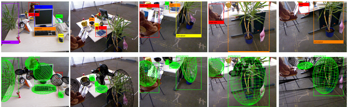
(1) C:20 , N_{in}:5 (6.4cm, 4.1°) error on \Theta_2 = 1.0^\circ (2) C:21 , N_{in}:3 (15.4cm, 3.6°) error on \Theta_2 = 2.3^\circ (3) C:29 , N_{in}:4 (21.1cm, 4.4°) error on \Theta_2 = 1.7^\circ (4) C:2 , N_{in}:2 (15.4cm, 7.6°) error on \Theta_2 = 6.1^\circ (5) C:3 , N_{in}:2 (263.0cm, 151.3°) error on \Theta_2 = 45.3^\circ
