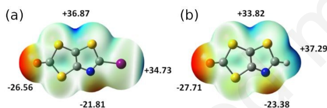
Fig. 3 Molecular electrostatic potential surfaces mapped at 0.001 e - .au -3 isodensity surface for (a) 2 ; (b) 3 . The common color scale ranges from -28 kcal.mol -1 (red) to +40 kcal.mol -1 (blue).
