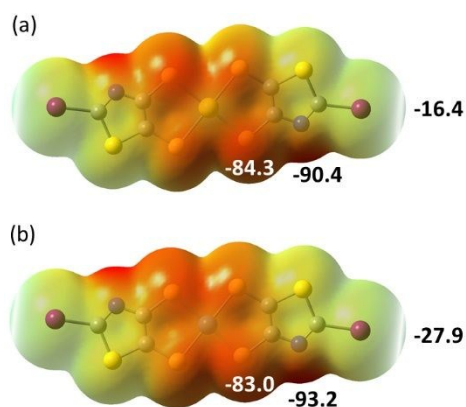
Fig. 8 Molecular electrostatic potential surfaces at the 0.001 \text{ e}^- \cdot \text{au}^{-3} isodensity level for the monoanionic complexes \text{trans}[\text{M}(\text{I-tzdt})_2]^{-1} with (a) \text{M} = \text{Au} ; (b), \text{M} = \text{Ni} . Colour scale ranges from +36.89 \text{ kcal} \cdot \text{mol}^{-1} (blue) to -93.16 \text{ kcal} \cdot \text{mol}^{-1} (red).
