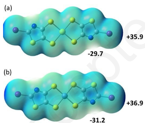
Fig. 9 Molecular electrostatic potential surfaces at the 0.001 \text{ e}^- \cdot \text{au}^{-3} isodensity level for the neutral complexes \text{trans}[\text{M}(\text{I-tzdt})_2] with (a) \text{M} = \text{Au} ; (b), \text{M} = \text{Ni} . Colour scale ranges from +36.89 \text{ kcal} \cdot \text{mol}^{-1} (blue) to -93.16 \text{ kcal} \cdot \text{mol}^{-1} (red).
