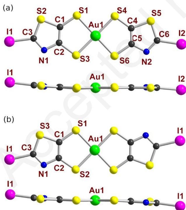
Fig. 5 Molecular view (top) and side view (bottom) of the monoanionic (a) cis - [\text{Au}(\text{I-tzdt})_2] and (b) trans - [\text{Au}(\text{I-tzdt})_2] complexes.
