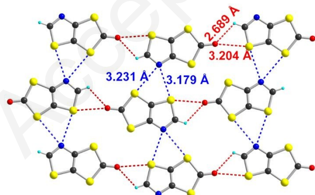
Fig. 2 Details of the shortest intermolecular H\cdots O , S\cdots O and S\cdots N contacts in 3 .
