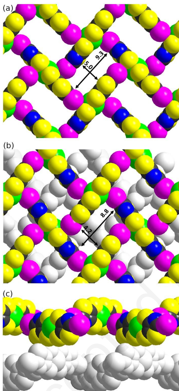
Fig. 7 (a) View of the solid state organization of trans -[Au(I-tzdt) 2 ] -1 anions with I...S XB interactions between complexes delineating channels. (b,c) Solid state organization of the cis -[Au(I-tzdt) 2 ] -1 anions with two alternating layers.
