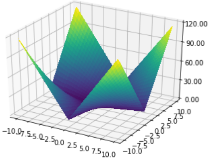
Figure 3: Schwefel 2 function: a simple piecewise linear function
