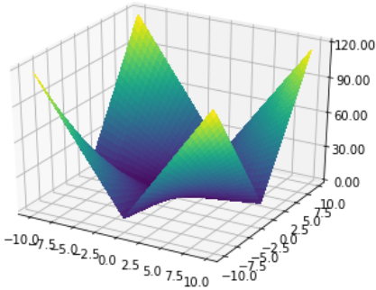
Figure 3: Schwefel 2 function: a simple piecewise linear function
