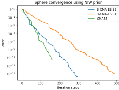
Figure 6: Convergence for the sphere function
