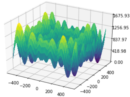
Figure 5: Schwefel 1 function: a non convex function multi-modal and with a large number of local pronounced bowls
