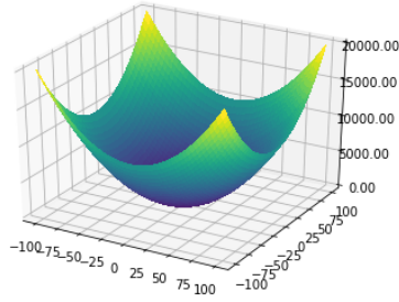
Figure 2: A simple convex function: the quadratic norm. Minimum in 0
