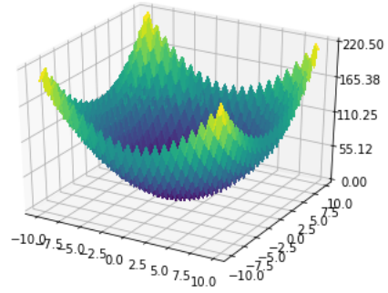
Figure 4: Rastrigin function: a non convex function multi-modal and with a large number of local minima
