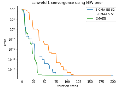
Figure 9: Convergence for the Schwefel 1 function
