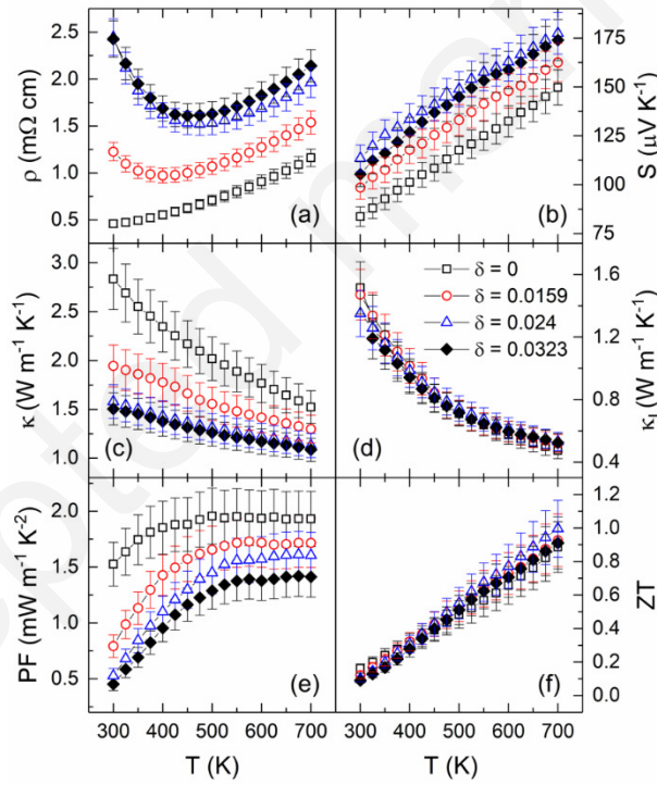
Figure 2. Temperature dependence of the (a) electrical resistivity ( \rho ), (b) Seebeck coefficient ( S ), (c) thermal conductivity ( \kappa ), (d) lattice thermal conductivity ( \kappa_L ), (e) power factor ( PF ), and (f) figure of merit ZT in the [\text{Cu}_{26}\text{Cr}_2\text{Ge}_6]_{1+\delta}\text{S}_{32} series.
