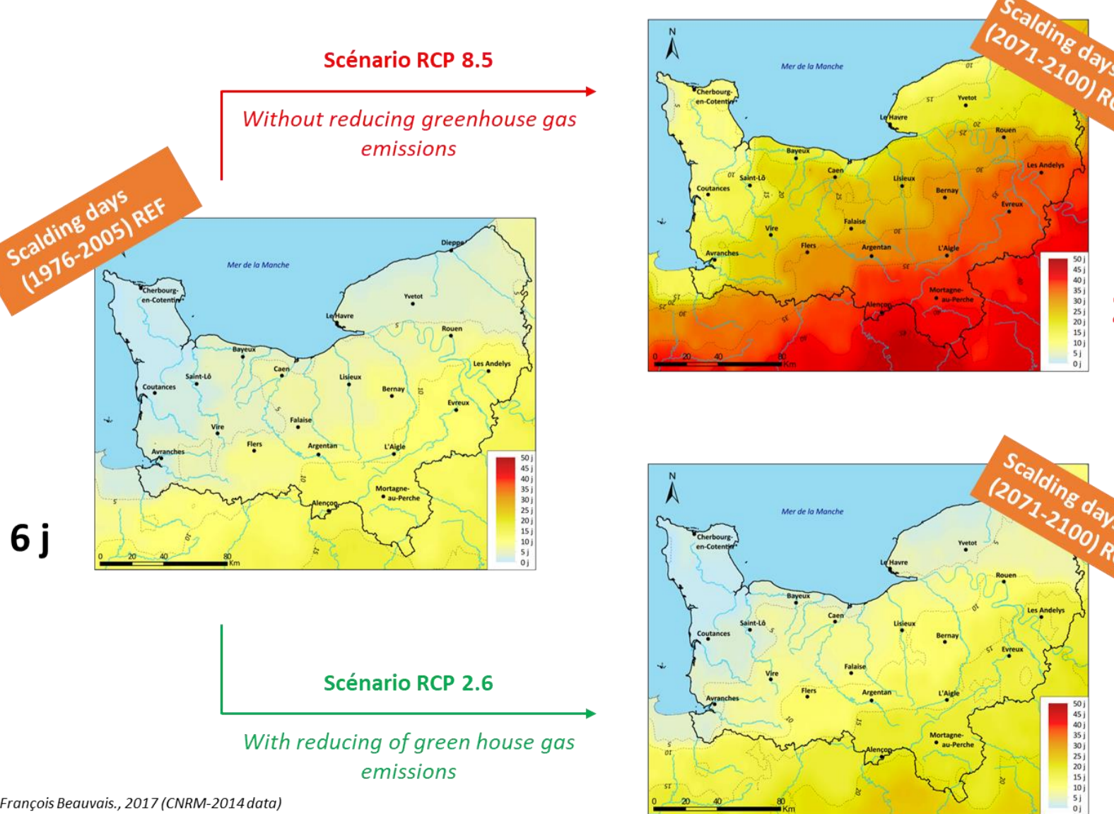
Fig.3 Evolution of scalding days (25°C) in May, June and July by 2100 in Normandy
