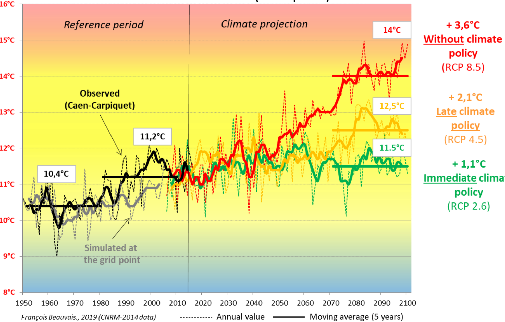
Fig.2 Evolution of the average annual temperature from 1950 to 2018 based on Caen-Carpique (weather station) data and CNRM-2014 data (ALADIN model) for a historical scenario (past period) and three RCP scenarios (future period) for Caen
