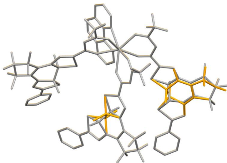
Figure S4. Simplified view of the crystal structure of 5ccc showing the two positions (50 % occupancy factor) of two of the DTE cores.
