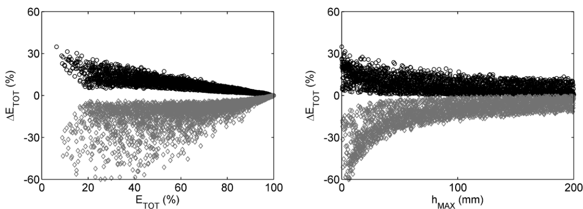
Figure 9. Percent deviations in E_{TOT} as function of E_{TOT} and h_{MAX} for the GA equation with fixed initial water content GA- \theta_{FC} (black circles) and the constant rate CR infiltration model (grey diamonds) (the figure associated with GA-RR can be found in supplementary materials)
