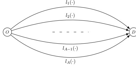
FIGURE 1. Example of a composite potential game
