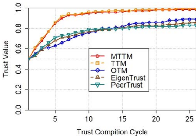
Fig. 14. Trust values of different derivatives of the algorithm and baseline schemes for randomly selected good fog server.
