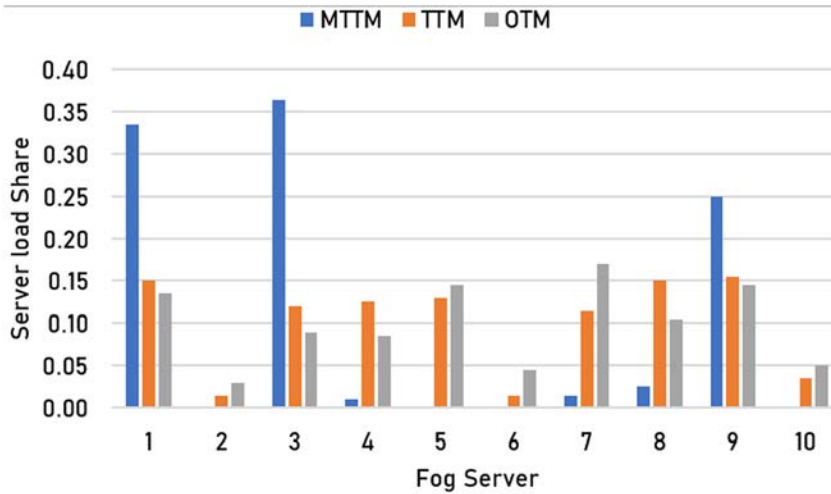
Fig. 13. Load distribution of randomly selected fog servers.
