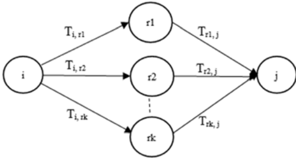
Fig. 5. Computation of overall indirect trust.
