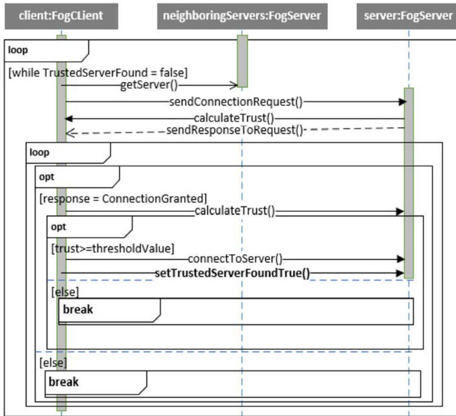
Fig. 2. Dialog between fog clients and fog servers.
