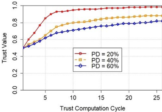
Fig. 8. Effect of percentage of bad nodes on trust values of a good fog client.
