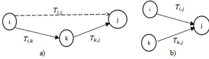
Fig. 4. (a) Discounting and (b) Consensus operators.
