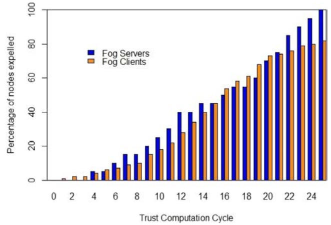
Fig. 9. Percentage of expelled bad nodes over trust computation cycle.
