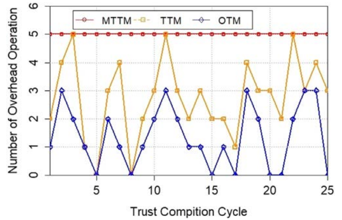
Fig. 12. Number of overhead operations over trust computation cycle.
