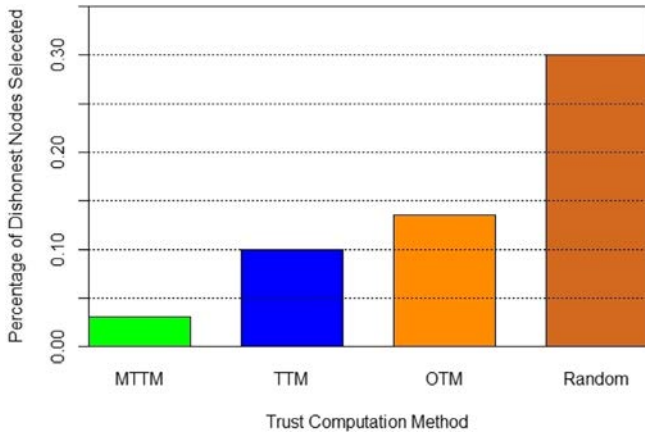
Fig. 11. Average percentage of bad fog servers selected for service provision.
